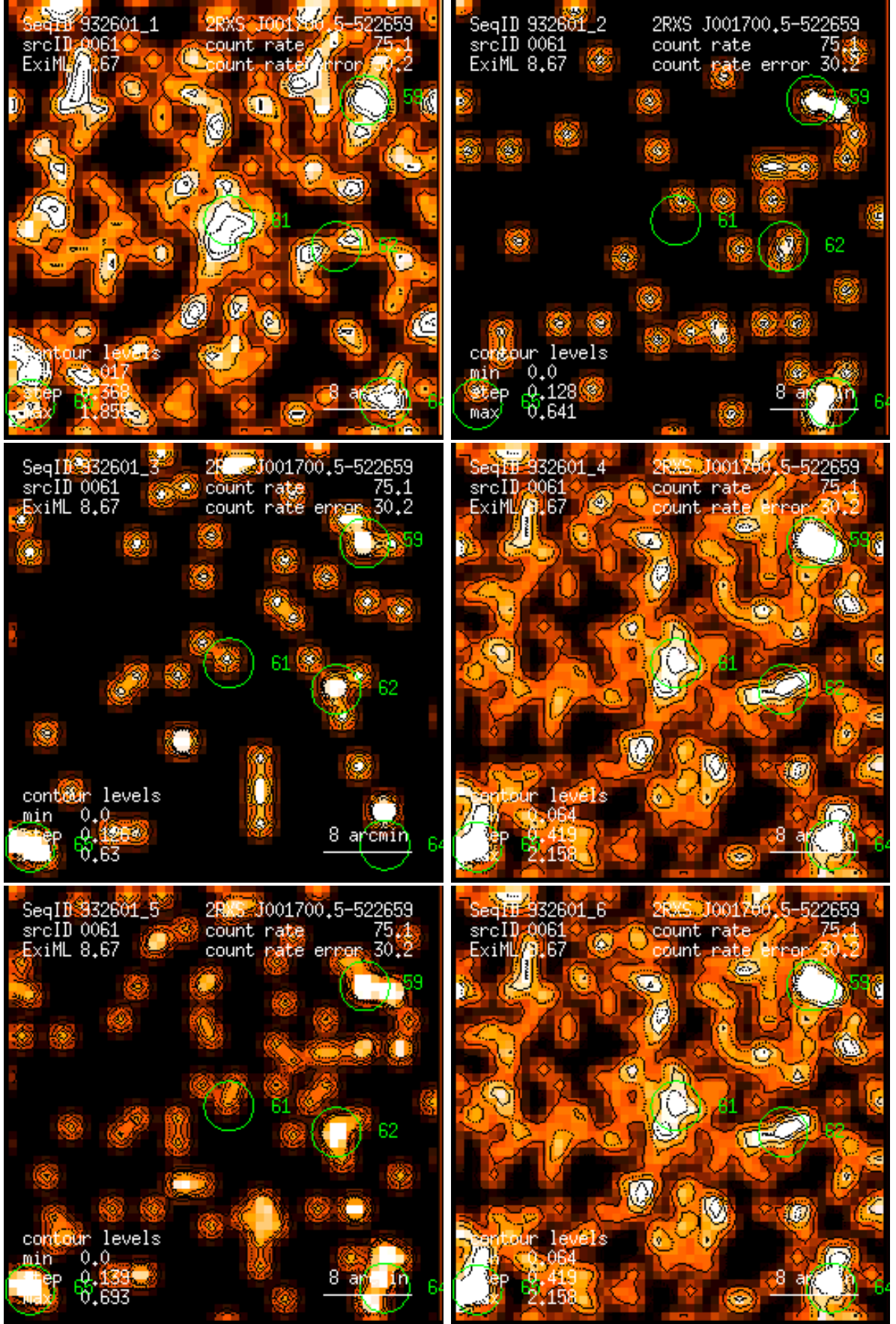
Figure 61: RASS 932601: detection 0061: band rate images, Gaussian filter: (1) PSPC channels 11 – 41, (2) 52 – 90, (3) 91 – 201, (4) 11 – 235, (5) 52 – 201, (6) 11 – 201. Broad band rates in counts/ks. Band rate contour levels in counts/ks/arcmin 2 .
