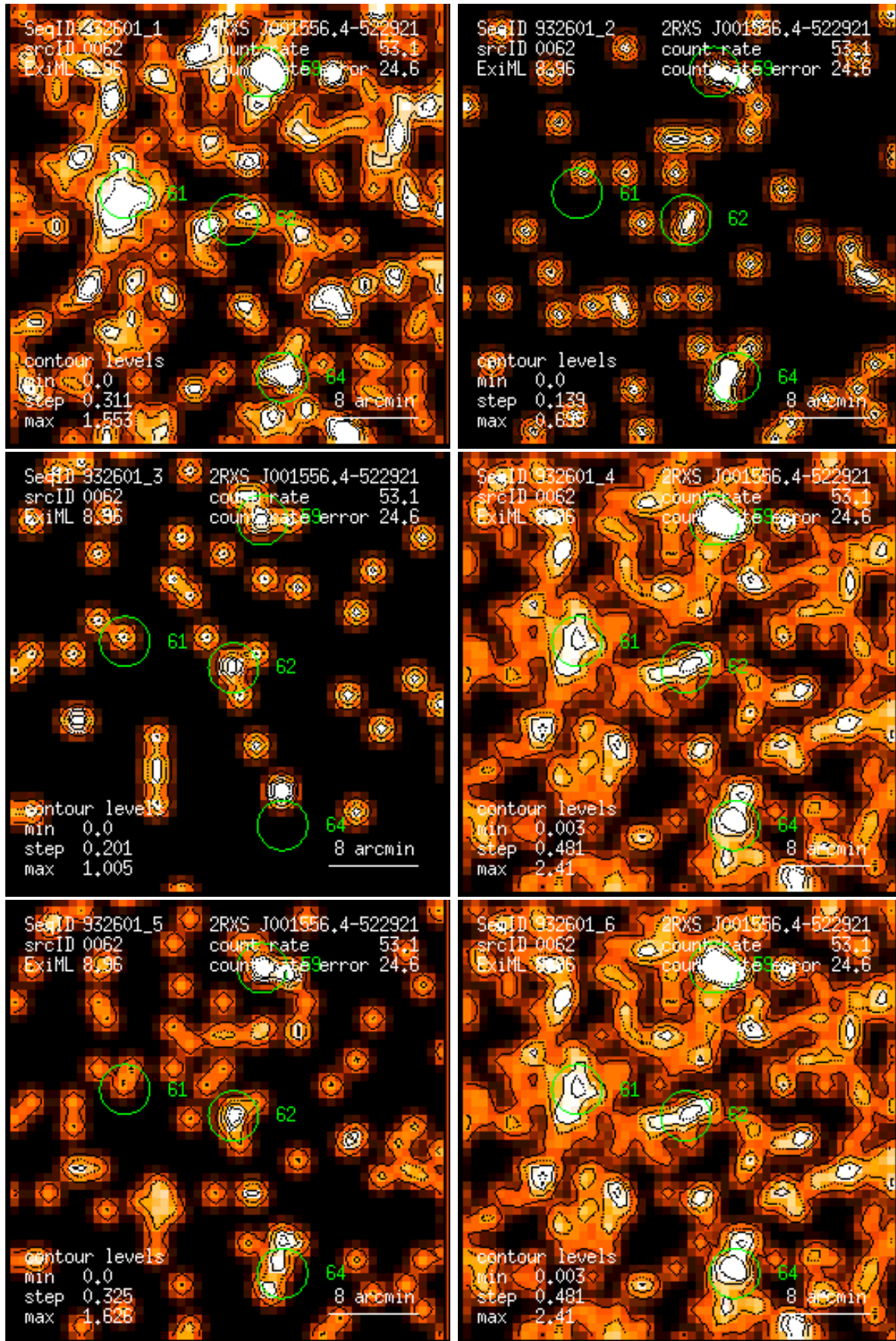
Figure 62: RASS 932601: detection 0062: band rate images, Gaussian filter: (1) PSPC channels 11 – 41, (2) 52 – 90, (3) 91 – 201, (4) 11 – 235, (5) 52 – 201, (6) 11 – 201. Broad band rates in counts/ks. Band rate contour levels in counts/ks/arcmin 2 .
