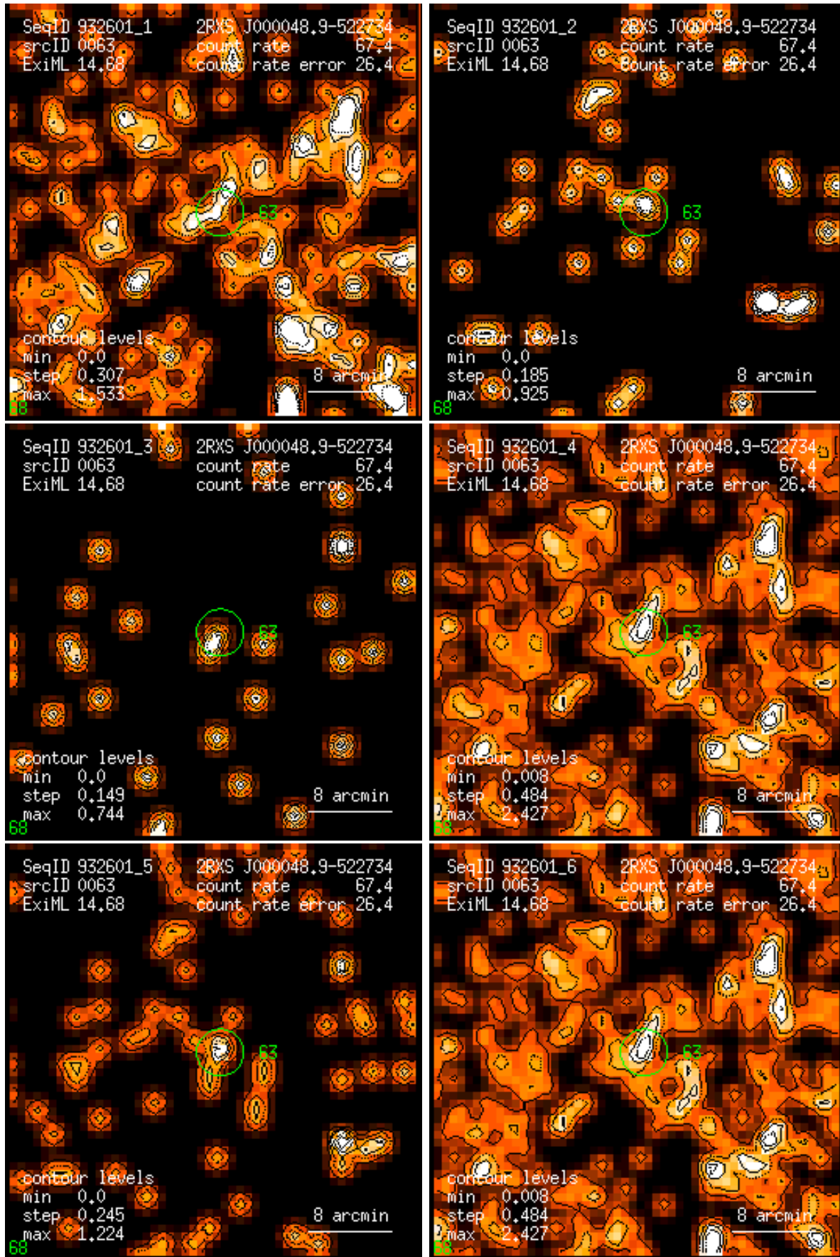
Figure 63: RASS 932601: detection 0063: band rate images, Gaussian filter: (1) PSPC channels 11 – 41, (2) 52 – 90, (3) 91 – 201, (4) 11 – 235, (5) 52 – 201, (6) 11 – 201. Broad band rates in counts/ks. Band rate contour levels in counts/ks/arcmin 2 .
