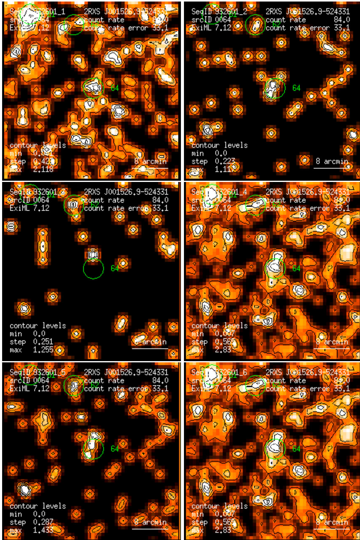
Figure 64: RASS 932601: detection 0064: band rate images, Gaussian filter: (1) PSPC channels 11 – 41, (2) 52 – 90, (3) 91 – 201, (4) 11 – 235, (5) 52 – 201, (6) 11 – 201. Broad band rates in counts/ks. Band rate contour levels in counts/ks/arcmin 2 .
