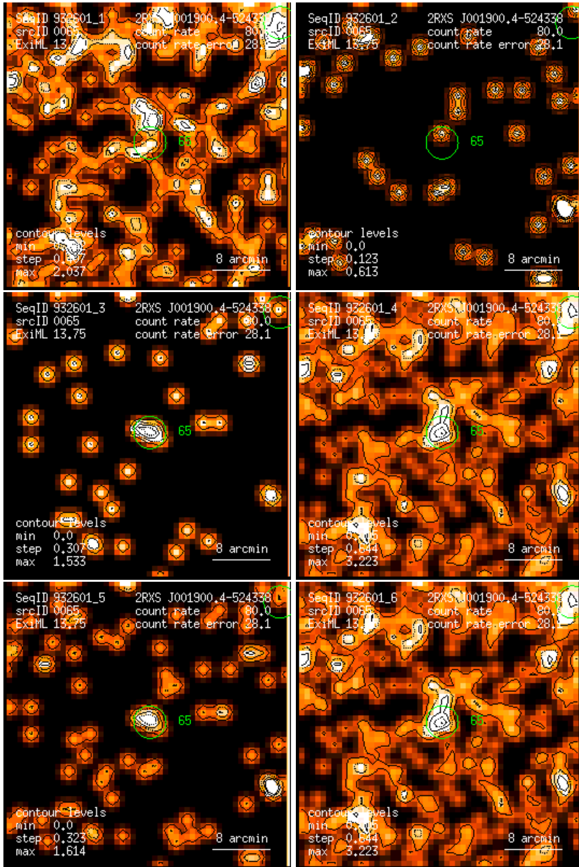
Figure 65: RASS 932601: detection 0065: band rate images, Gaussian filter: (1) PSPC channels 11 – 41, (2) 52 – 90, (3) 91 – 201, (4) 11 – 235, (5) 52 – 201, (6) 11 – 201. Broad band rates in counts/ks. Band rate contour levels in counts/ks/arcmin 2 .
