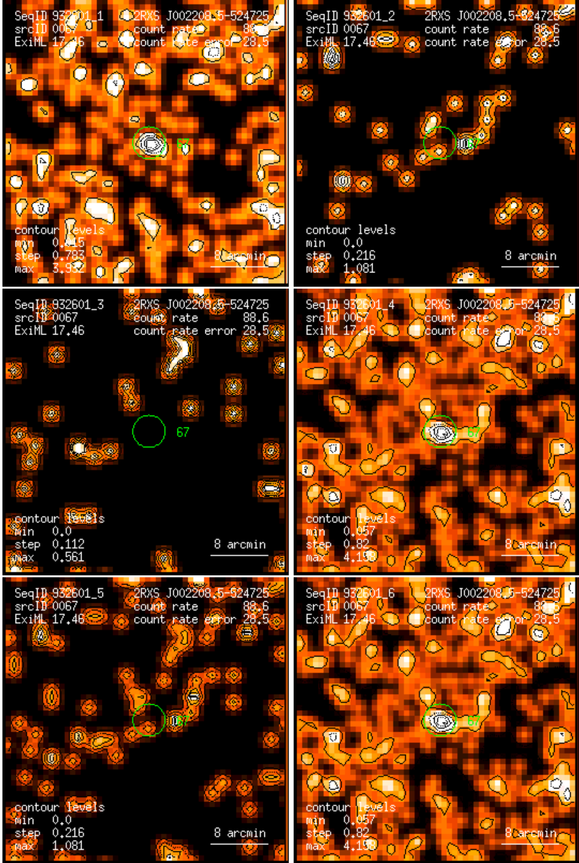
Figure 67: RASS 932601: detection 0067: band rate images, Gaussian filter: (1) PSPC channels 11 – 41, (2) 52 – 90, (3) 91 – 201, (4) 11 – 235, (5) 52 – 201, (6) 11 – 201. Broad band rates in counts/ks. Band rate contour levels in counts/ks/arcmin 2 .
