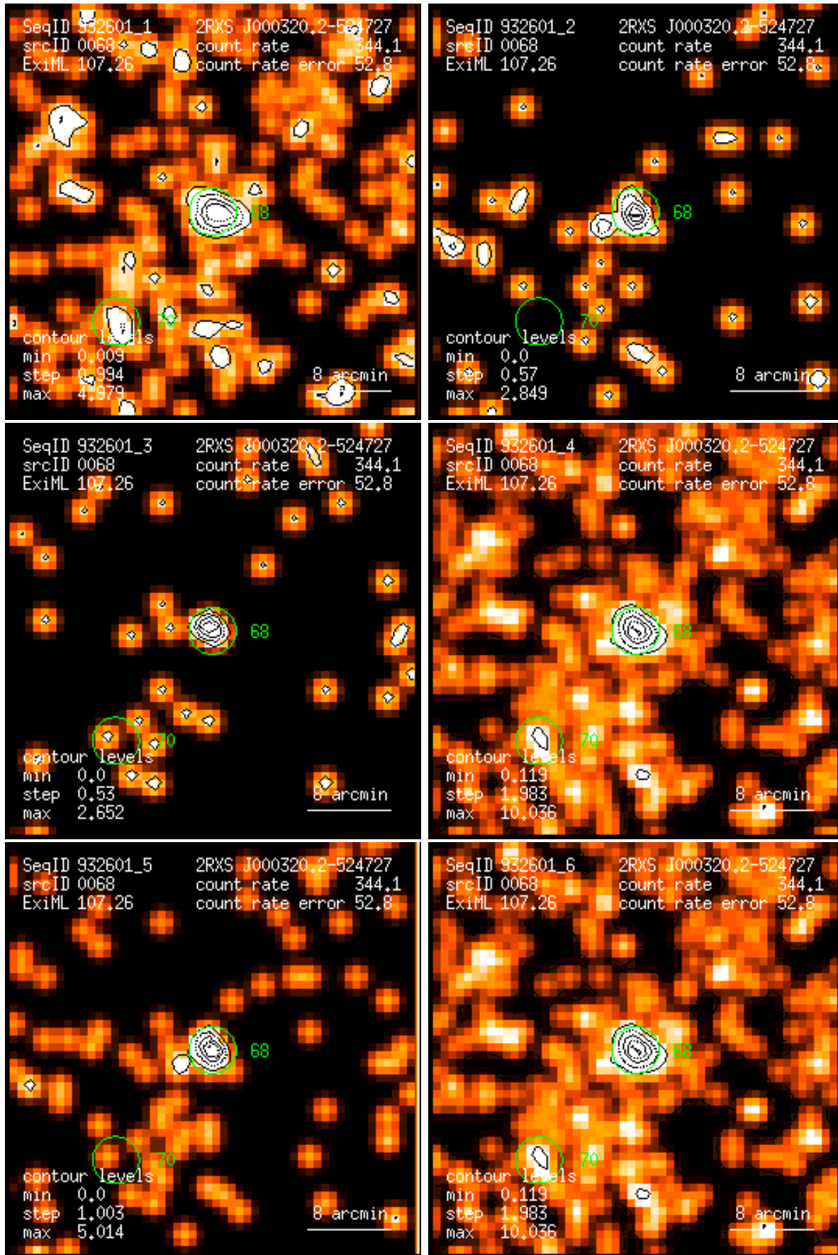
Figure 68: RASS 932601: detection 0068: band rate images, Gaussian filter: (1) PSPC channels 11 – 41, (2) 52 – 90, (3) 91 – 201, (4) 11 – 235, (5) 52 – 201, (6) 11 – 201. Broad band rates in counts/ks. Band rate contour levels in counts/ks/arcmin 2 .
