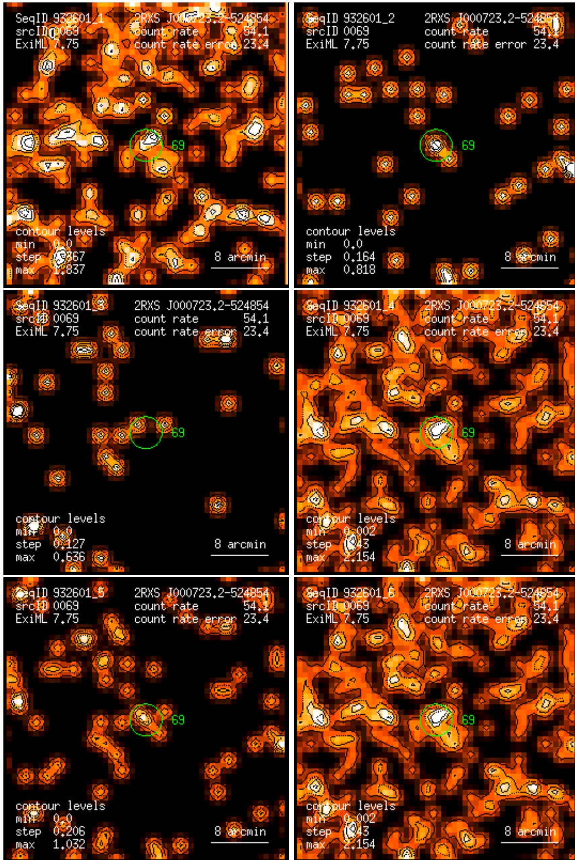
Figure 69: RASS 932601: detection 0069: band rate images, Gaussian filter: (1) PSPC channels 11 – 41, (2) 52 – 90, (3) 91 – 201, (4) 11 – 235, (5) 52 – 201, (6) 11 – 201. Broad band rates in counts/ks. Band rate contour levels in counts/ks/arcmin 2 .
