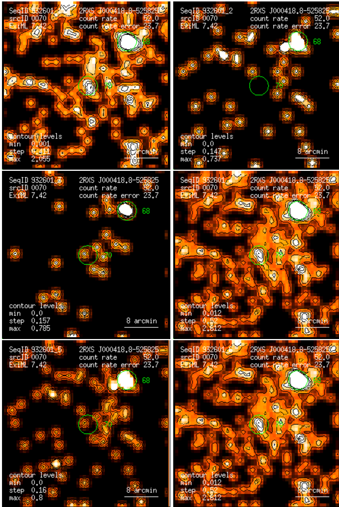
Figure 70: RASS 932601: detection 0070: band rate images, Gaussian filter: (1) PSPC channels 11 – 41, (2) 52 – 90, (3) 91 – 201, (4) 11 – 235, (5) 52 – 201, (6) 11 – 201. Broad band rates in counts/ks. Band rate contour levels in counts/ks/arcmin 2 .
