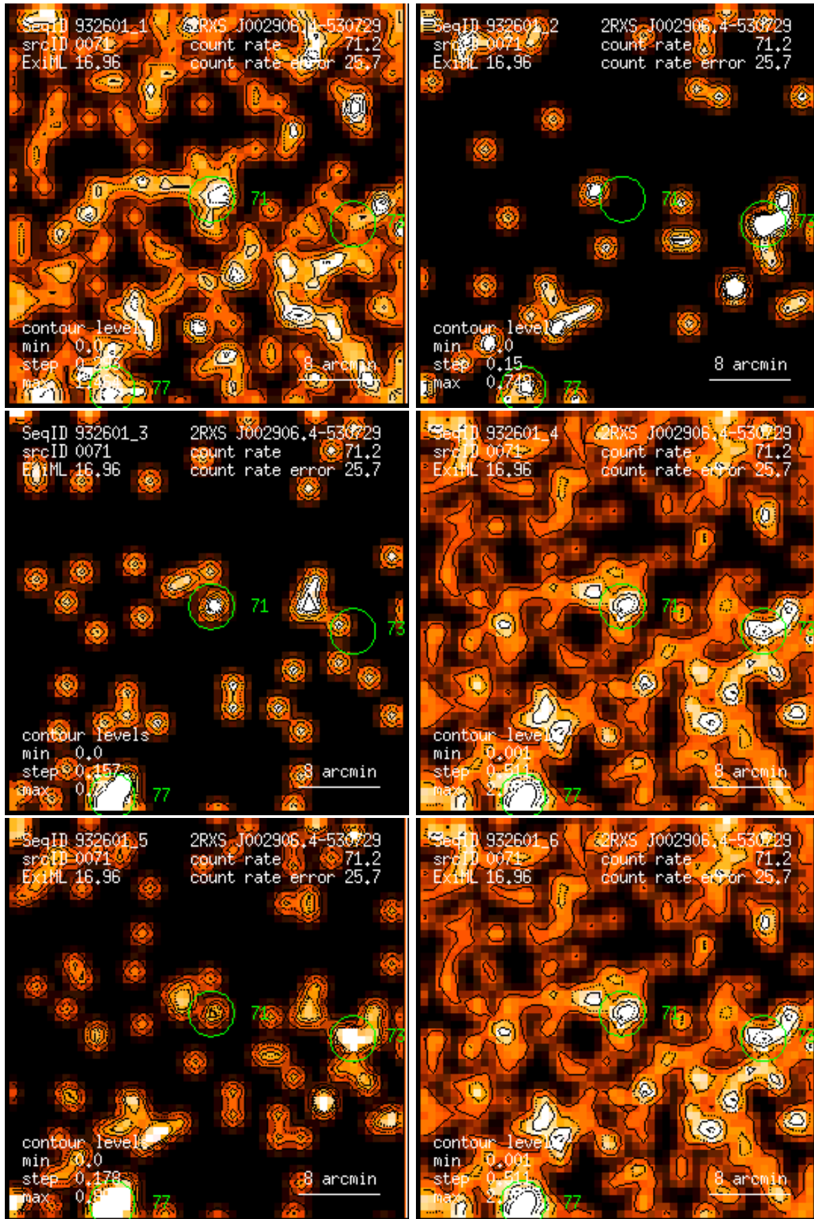
Figure 71: RASS 932601: detection 0071: band rate images, Gaussian filter: (1) PSPC channels 11 – 41, (2) 52 – 90, (3) 91 – 201, (4) 11 – 235, (5) 52 – 201, (6) 11 – 201. Broad band rates in counts/ks. Band rate contour levels in counts/ks/arcmin 2 .
