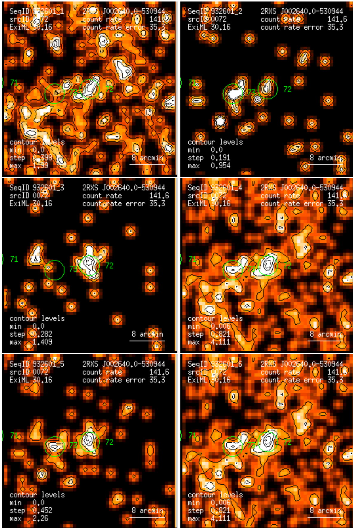
Figure 72: RASS 932601: detection 0072: band rate images, Gaussian filter: (1) PSPC channels 11 – 41, (2) 52 – 90, (3) 91 – 201, (4) 11 – 235, (5) 52 – 201, (6) 11 – 201. Broad band rates in counts/ks. Band rate contour levels in counts/ks/arcmin 2 .
