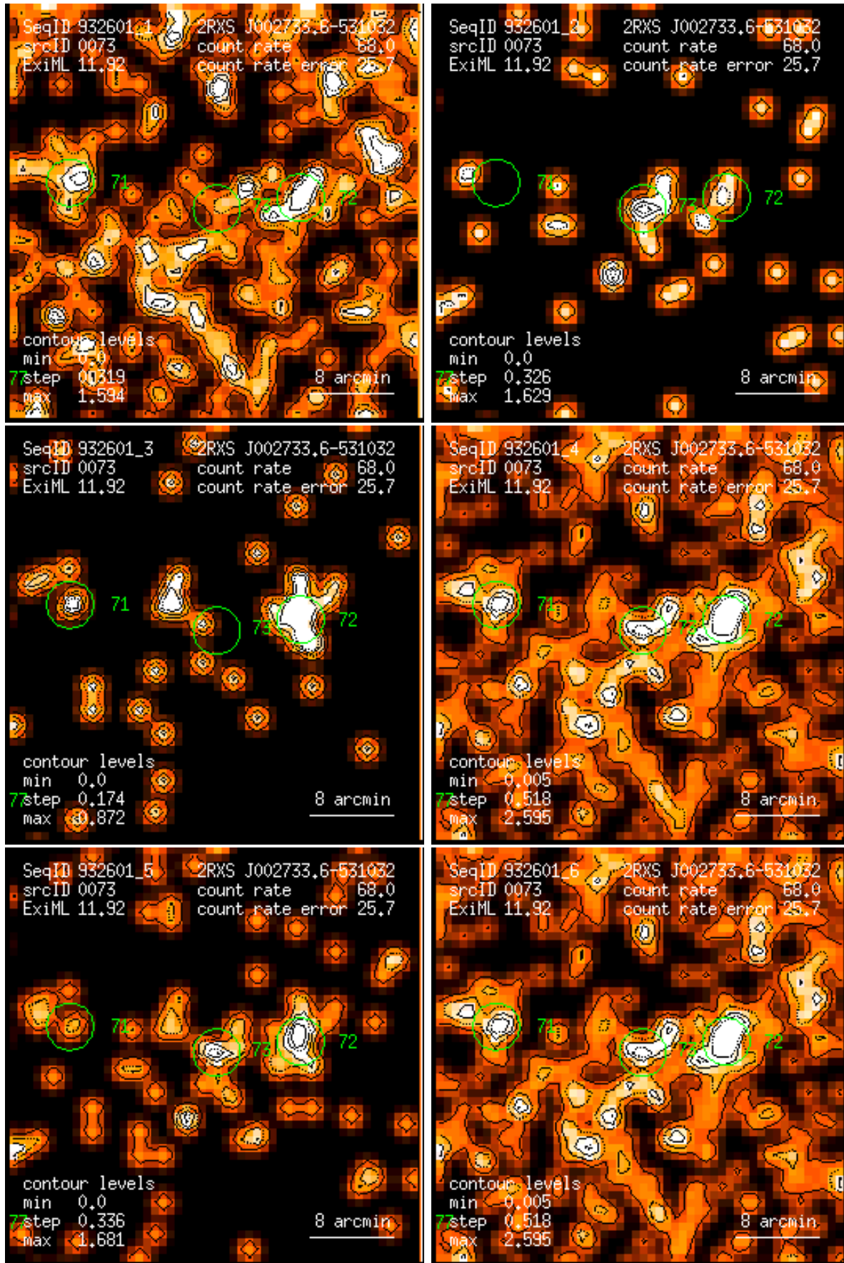
Figure 73: RASS 932601: detection 0073: band rate images, Gaussian filter: (1) PSPC channels 11 – 41, (2) 52 – 90, (3) 91 – 201, (4) 11 – 235, (5) 52 – 201, (6) 11 – 201. Broad band rates in counts/ks. Band rate contour levels in counts/ks/arcmin 2 .
