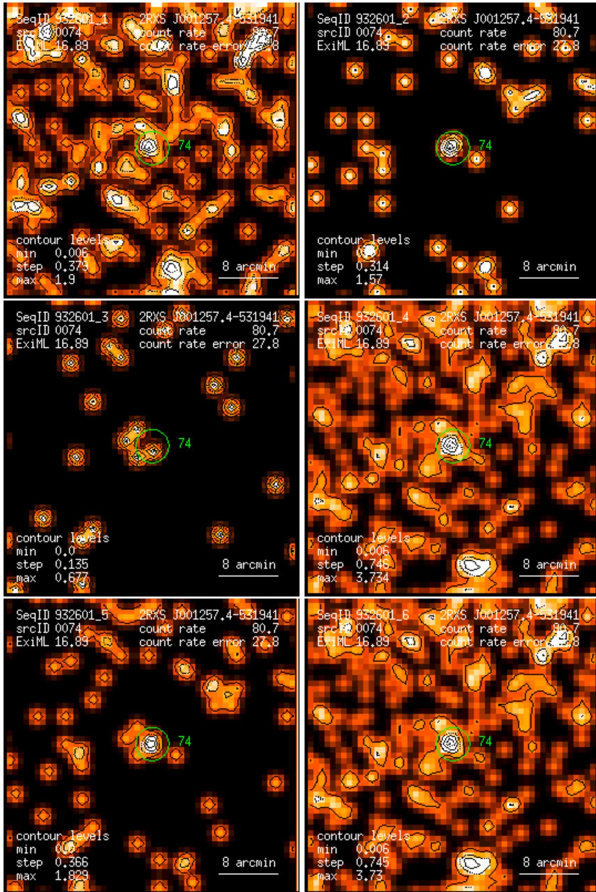
Figure 74: RASS 932601: detection 0074: band rate images, Gaussian filter: (1) PSPC channels 11 – 41, (2) 52 – 90, (3) 91 – 201, (4) 11 – 235, (5) 52 – 201, (6) 11 – 201. Broad band rates in counts/ks. Band rate contour levels in counts/ks/arcmin 2 .
