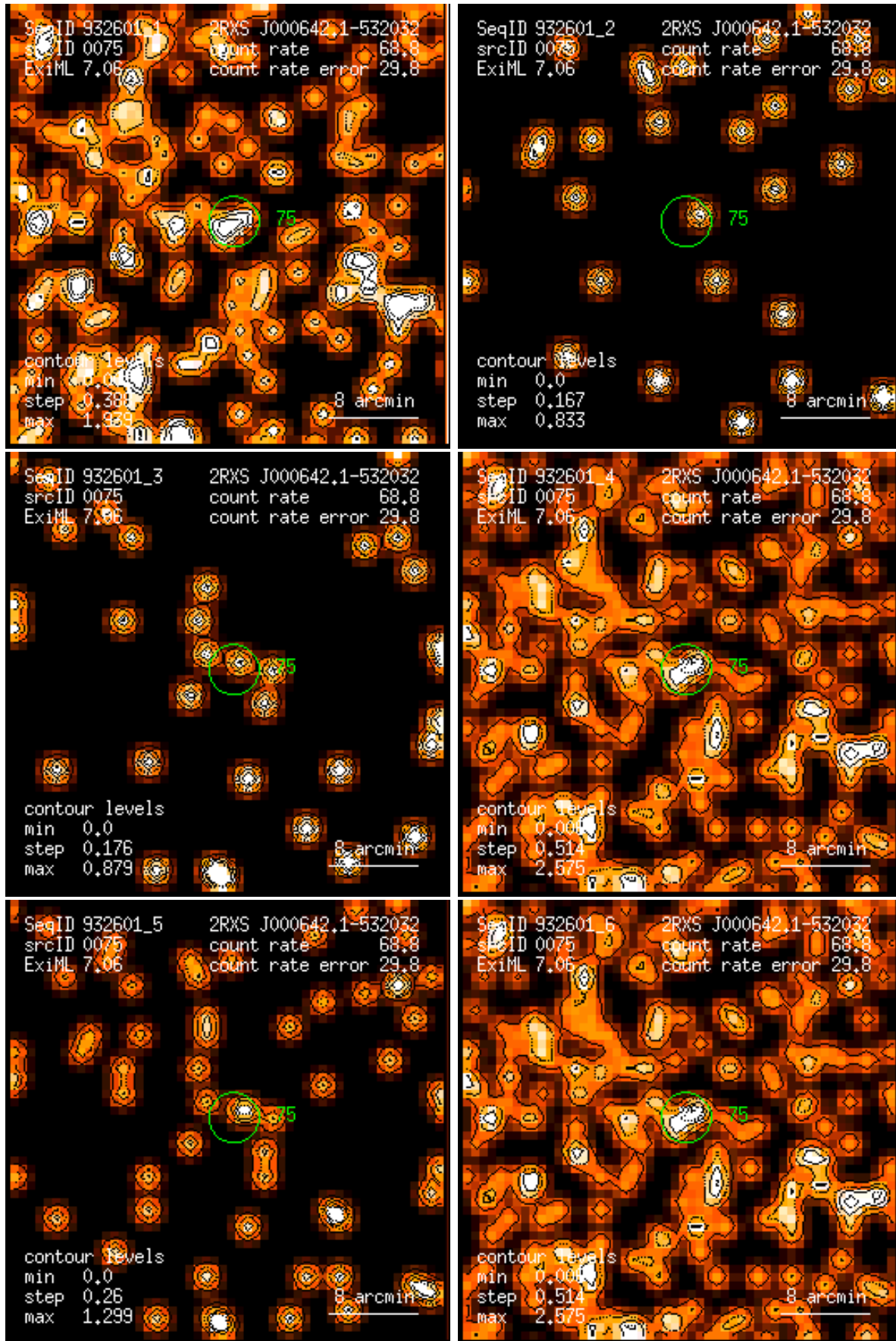
Figure 75: RASS 932601: detection 0075: band rate images, Gaussian filter: (1) PSPC channels 11 – 41, (2) 52 – 90, (3) 91 – 201, (4) 11 – 235, (5) 52 – 201, (6) 11 – 201. Broad band rates in counts/ks. Band rate contour levels in counts/ks/arcmin 2 .
