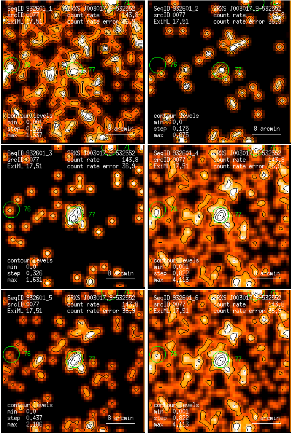
Figure 77: RASS 932601: detection 0077: band rate images, Gaussian filter: (1) PSPC channels 11 – 41, (2) 52 – 90, (3) 91 – 201, (4) 11 – 235, (5) 52 – 201, (6) 11 – 201. Broad band rates in counts/ks. Band rate contour levels in counts/ks/arcmin 2 .
