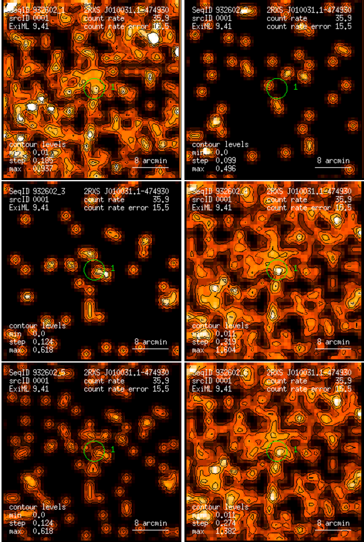
Figure 1: RASS 932602: detection 0001: band rate images, Gaussian filter: (1) PSPC channels 11 – 41, (2) 52 – 90, (3) 91 – 201, (4) 11 – 235, (5) 52 – 201, (6) 11 – 201. Broad band rates in counts/ks. Band rate contour levels in counts/ks/arcmin 2 .
