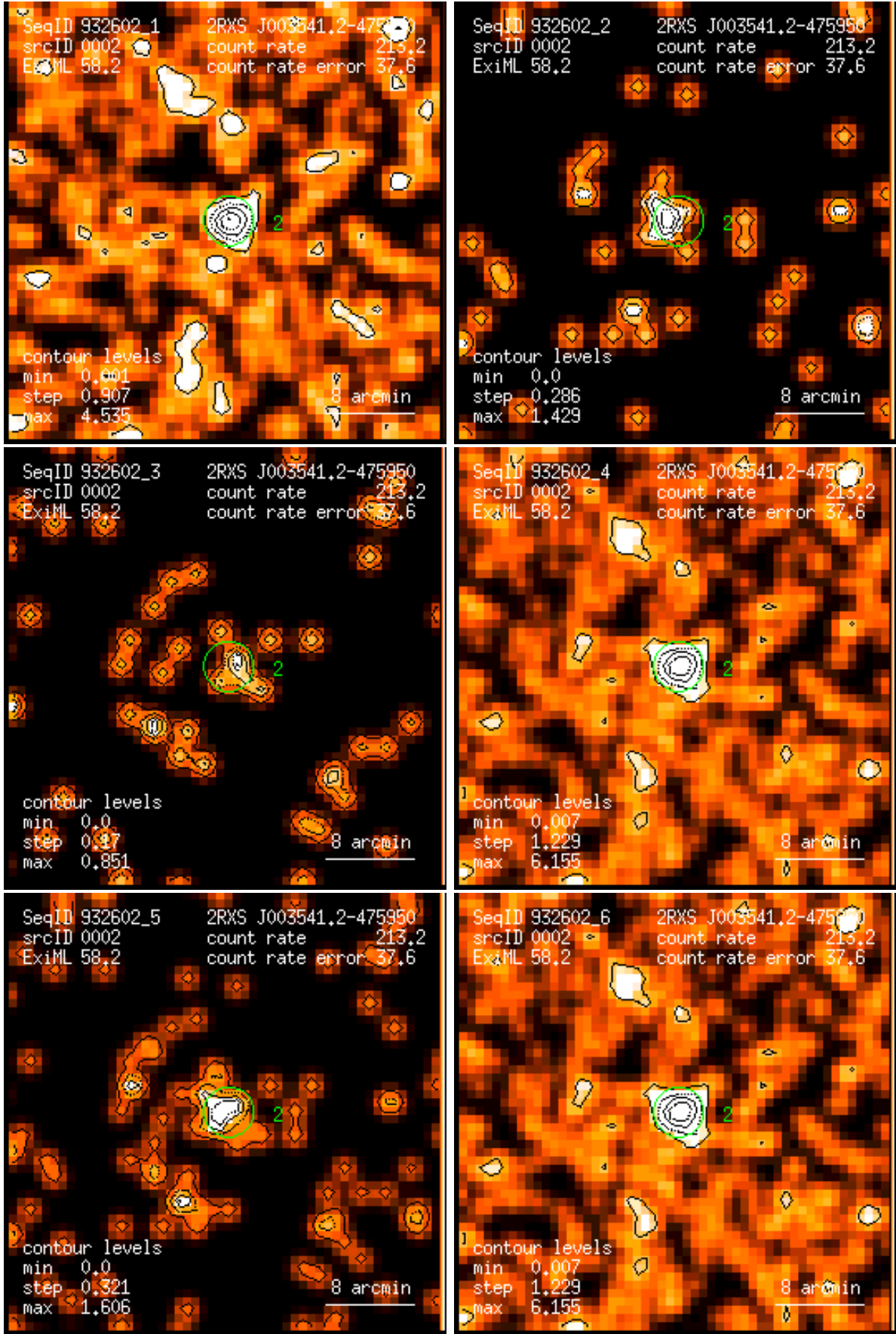
Figure 2: RASS 932602: detection 0002: band rate images, Gaussian filter: (1) PSPC channels 11 – 41, (2) 52 – 90, (3) 91 – 201, (4) 11 – 235, (5) 52 – 201, (6) 11 – 201. Broad band rates in counts/ks. Band rate contour levels in counts/ks/arcmin 2 .
