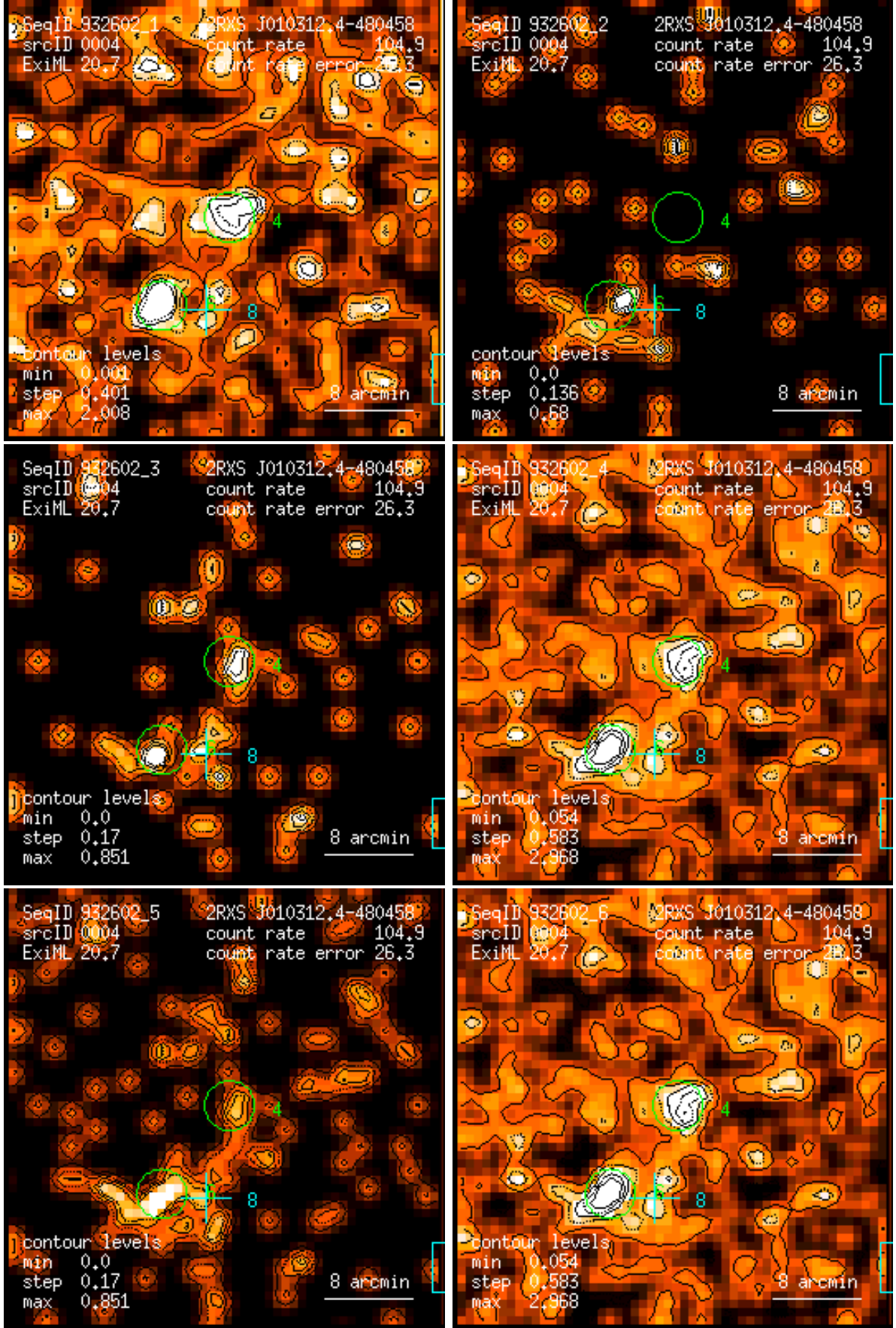
Figure 4: RASS 932602: detection 0004: band rate images, Gaussian filter: (1) PSPC channels 11 – 41, (2) 52 – 90, (3) 91 – 201, (4) 11 – 235, (5) 52 – 201, (6) 11 – 201. Broad band rates in counts/ks. Band rate contour levels in counts/ks/arcmin 2 .
