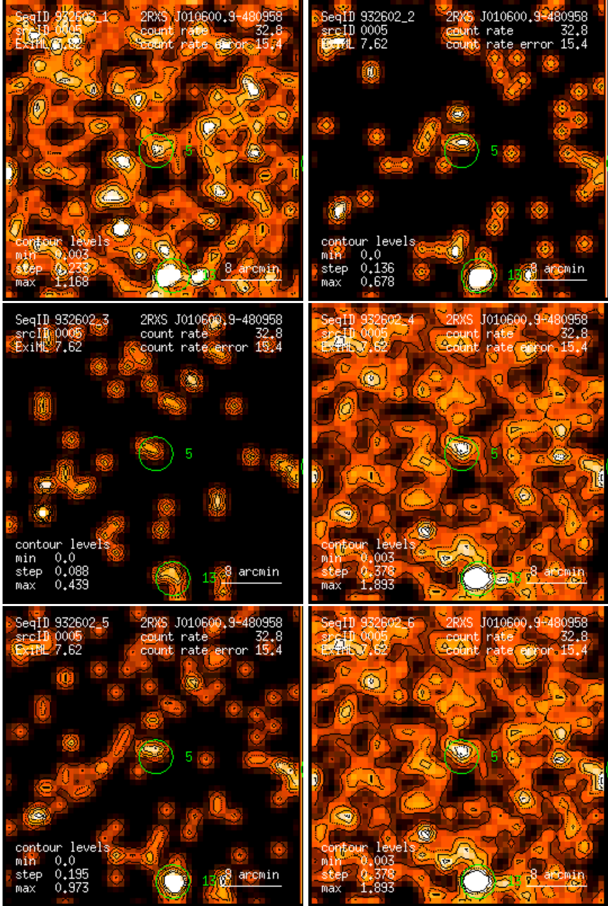
Figure 5: RASS 932602: detection 0005: band rate images, Gaussian filter: (1) PSPC channels 11 – 41, (2) 52 – 90, (3) 91 – 201, (4) 11 – 235, (5) 52 – 201, (6) 11 – 201. Broad band rates in counts/ks. Band rate contour levels in counts/ks/arcmin 2 .
