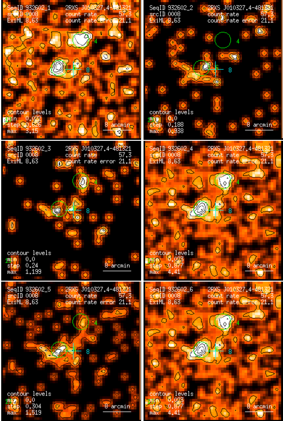
Figure 8: RASS 932602: detection 0008: band rate images, Gaussian filter: (1) PSPC channels 11 – 41, (2) 52 – 90, (3) 91 – 201, (4) 11 – 235, (5) 52 – 201, (6) 11 – 201. Broad band rates in counts/ks. Band rate contour levels in counts/ks/arcmin 2 .
