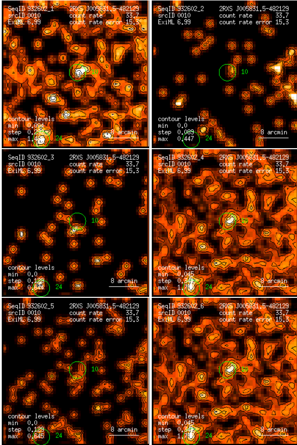
Figure 10: RASS 932602: detection 0010: band rate images, Gaussian filter: (1) PSPC channels 11 – 41, (2) 52 – 90, (3) 91 – 201, (4) 11 – 235, (5) 52 – 201, (6) 11 – 201. Broad band rates in counts/ks. Band rate contour levels in counts/ks/arcmin 2 .
