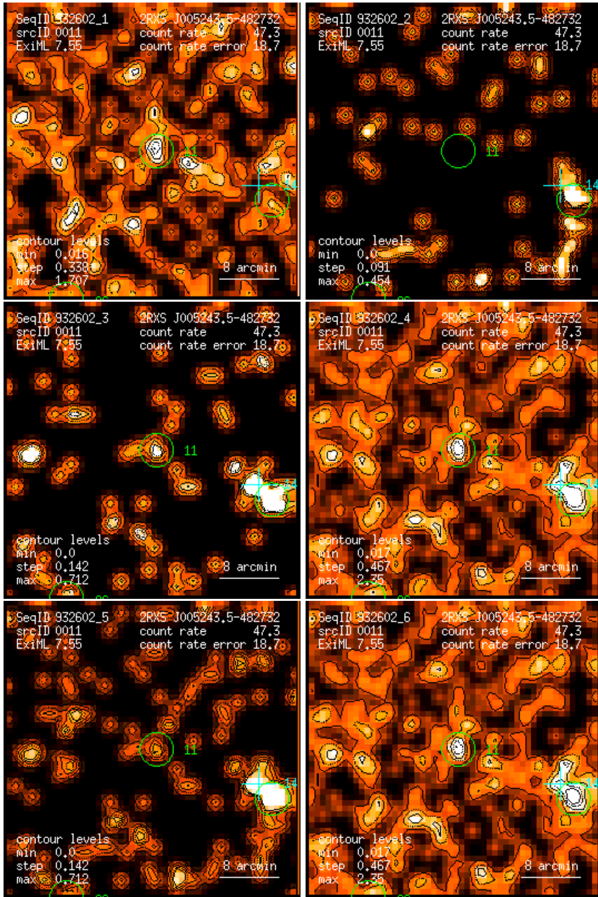
Figure 11: RASS 932602: detection 0011: band rate images, Gaussian filter: (1) PSPC channels 11 – 41, (2) 52 – 90, (3) 91 – 201, (4) 11 – 235, (5) 52 – 201, (6) 11 – 201. Broad band rates in counts/ks. Band rate contour levels in counts/ks/arcmin 2 .
