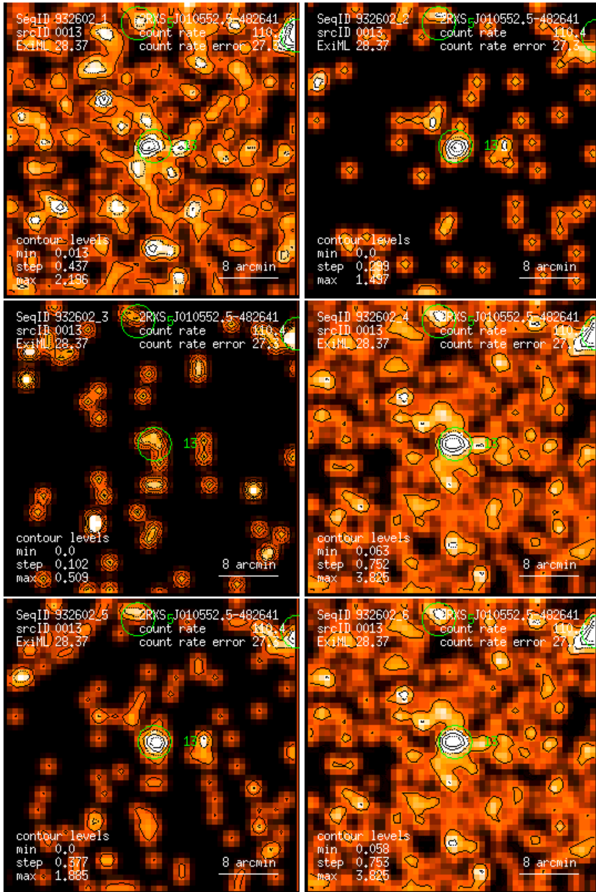
Figure 13: RASS 932602: detection 0013: band rate images, Gaussian filter: (1) PSPC channels 11 – 41, (2) 52 – 90, (3) 91 – 201, (4) 11 – 235, (5) 52 – 201, (6) 11 – 201. Broad band rates in counts/ks. Band rate contour levels in counts/ks/arcmin 2 .
