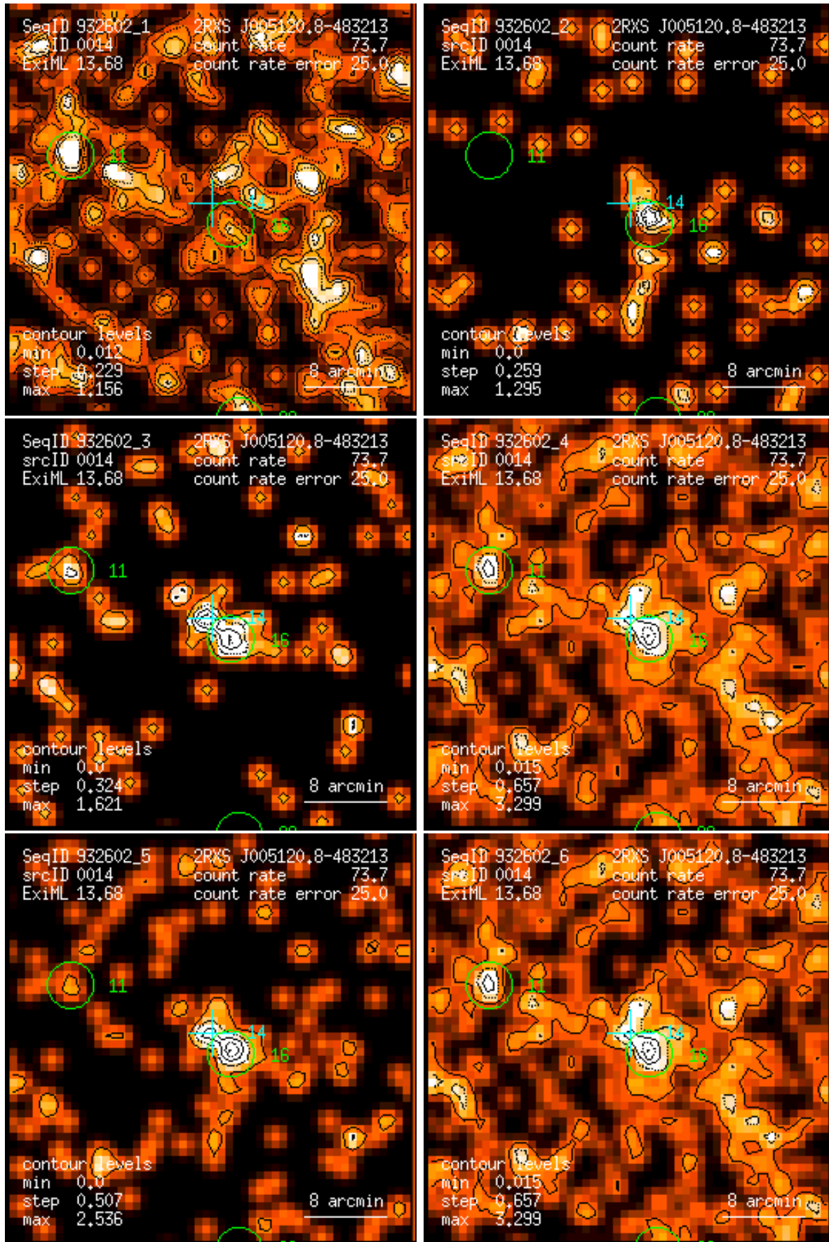
Figure 14: RASS 932602: detection 0014: band rate images, Gaussian filter: (1) PSPC channels 11 – 41, (2) 52 – 90, (3) 91 – 201, (4) 11 – 235, (5) 52 – 201, (6) 11 – 201. Broad band rates in counts/ks. Band rate contour levels in counts/ks/arcmin 2 .
