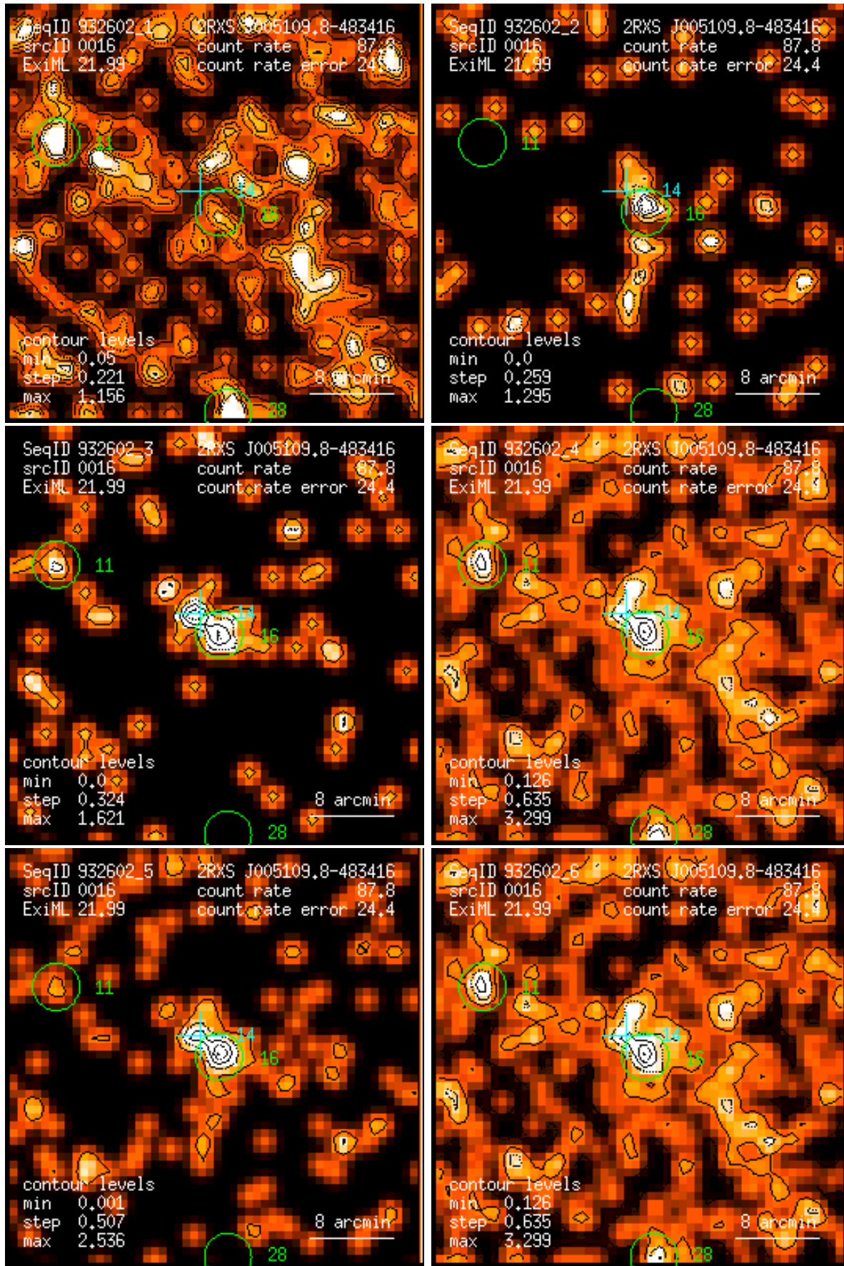
Figure 16: RASS 932602: detection 0016: band rate images, Gaussian filter: (1) PSPC channels 11 – 41, (2) 52 – 90, (3) 91 – 201, (4) 11 – 235, (5) 52 – 201, (6) 11 – 201. Broad band rates in counts/ks. Band rate contour levels in counts/ks/arcmin 2 .
