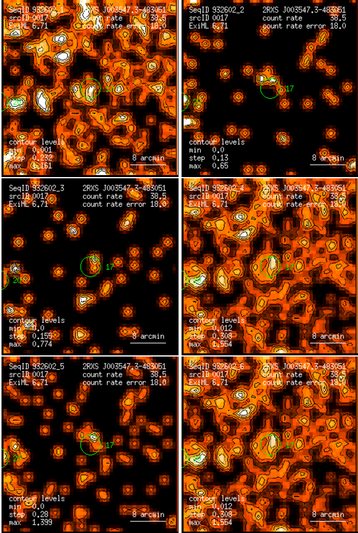
Figure 17: RASS 932602: detection 0017: band rate images, Gaussian filter: (1) PSPC channels 11 – 41, (2) 52 – 90, (3) 91 – 201, (4) 11 – 235, (5) 52 – 201, (6) 11 – 201. Broad band rates in counts/ks. Band rate contour levels in counts/ks/arcmin 2 .
