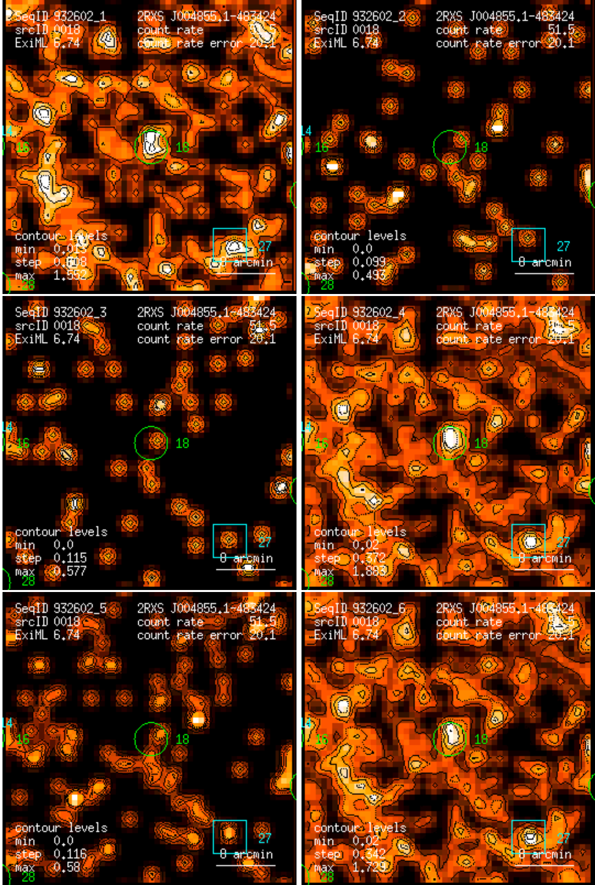
Figure 18: RASS 932602: detection 0018: band rate images, Gaussian filter: (1) PSPC channels 11 – 41, (2) 52 – 90, (3) 91 – 201, (4) 11 – 235, (5) 52 – 201, (6) 11 – 201. Broad band rates in counts/ks. Band rate contour levels in counts/ks/arcmin 2 .
