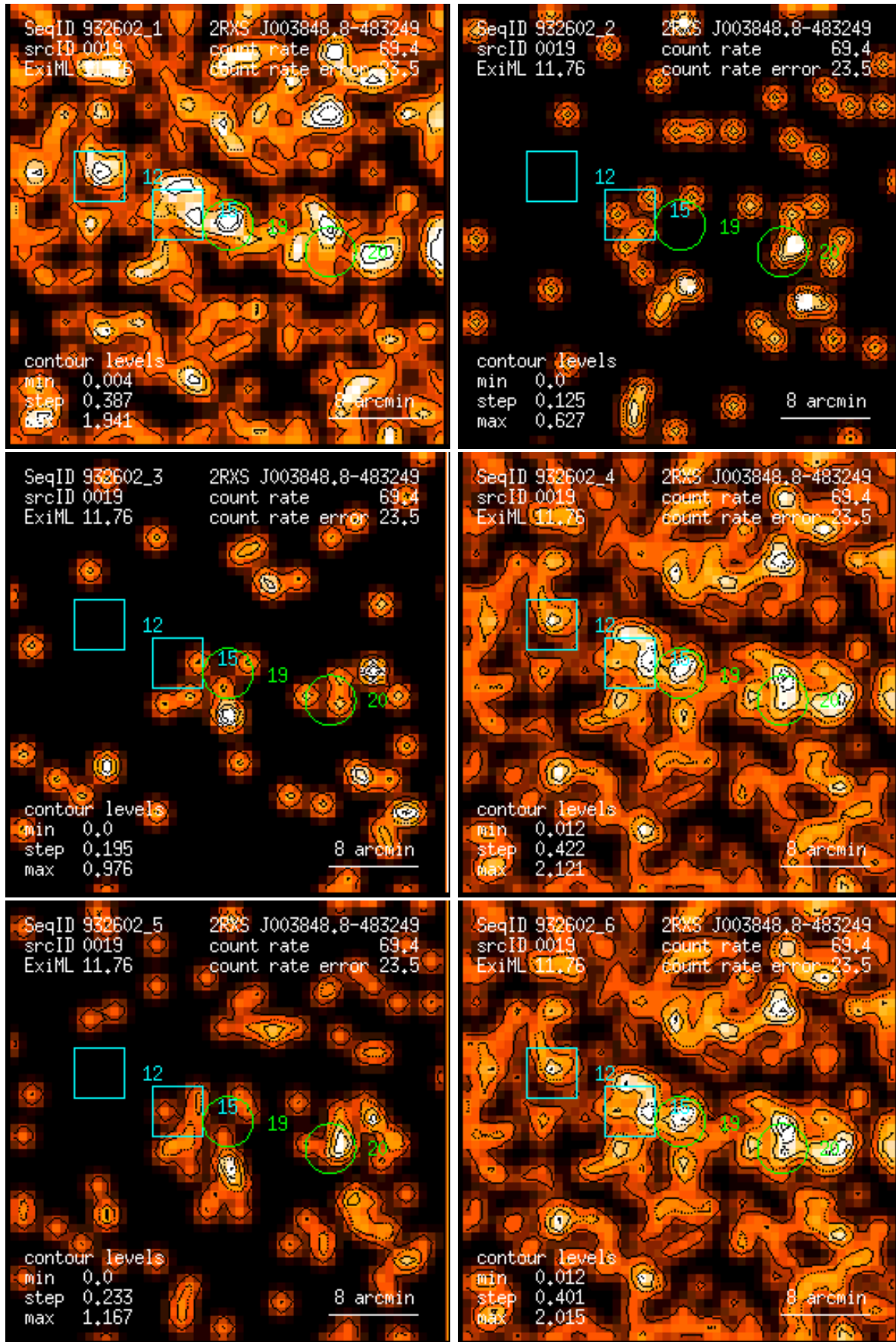
Figure 19: RASS 932602: detection 0019: band rate images, Gaussian filter: (1) PSPC channels 11 – 41, (2) 52 – 90, (3) 91 – 201, (4) 11 – 235, (5) 52 – 201, (6) 11 – 201. Broad band rates in counts/ks. Band rate contour levels in counts/ks/arcmin 2 .
