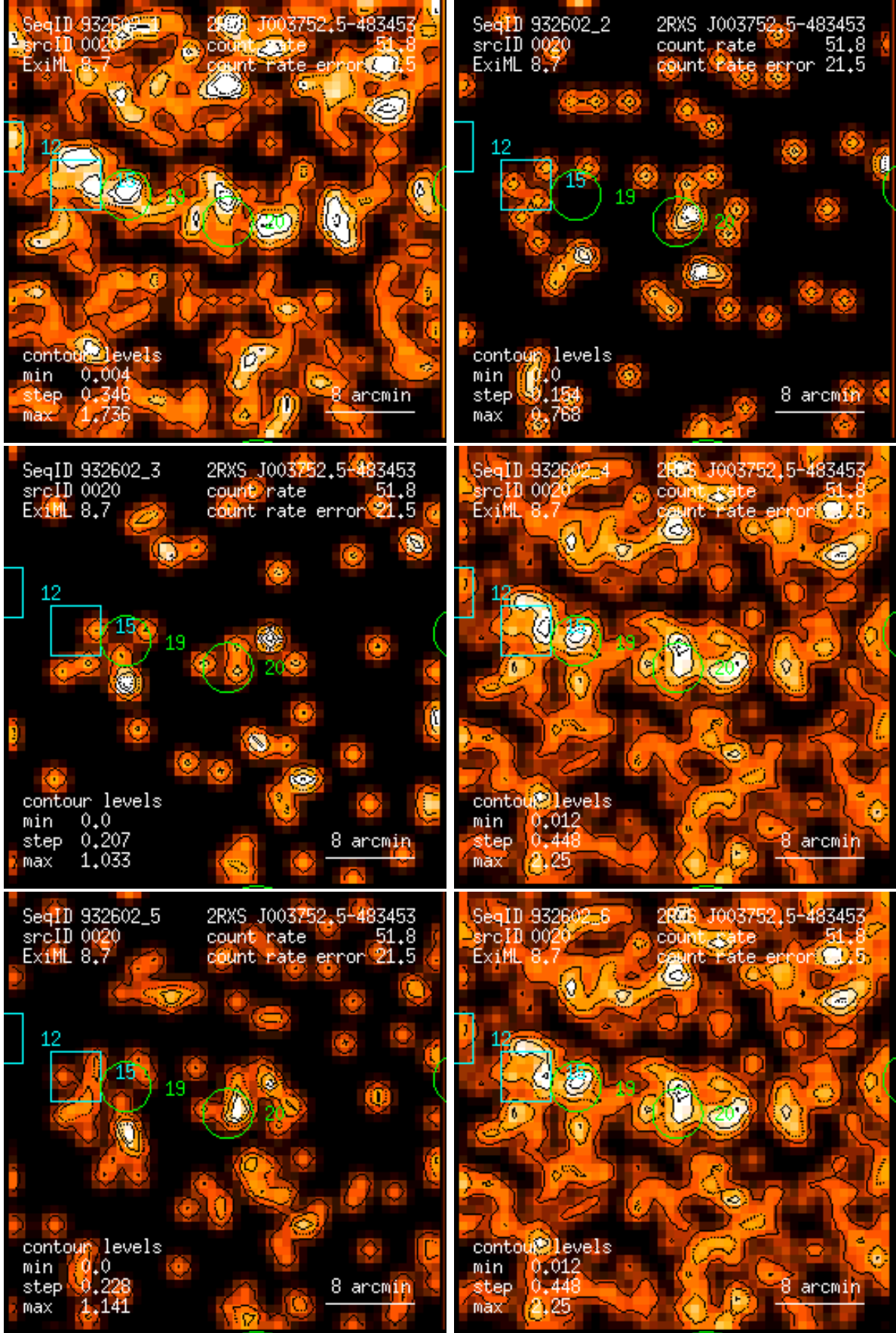
Figure 20: RASS 932602: detection 0020: band rate images, Gaussian filter: (1) PSPC channels 11 – 41, (2) 52 – 90, (3) 91 – 201, (4) 11 – 235, (5) 52 – 201, (6) 11 – 201. Broad band rates in counts/ks. Band rate contour levels in counts/ks/arcmin 2 .
