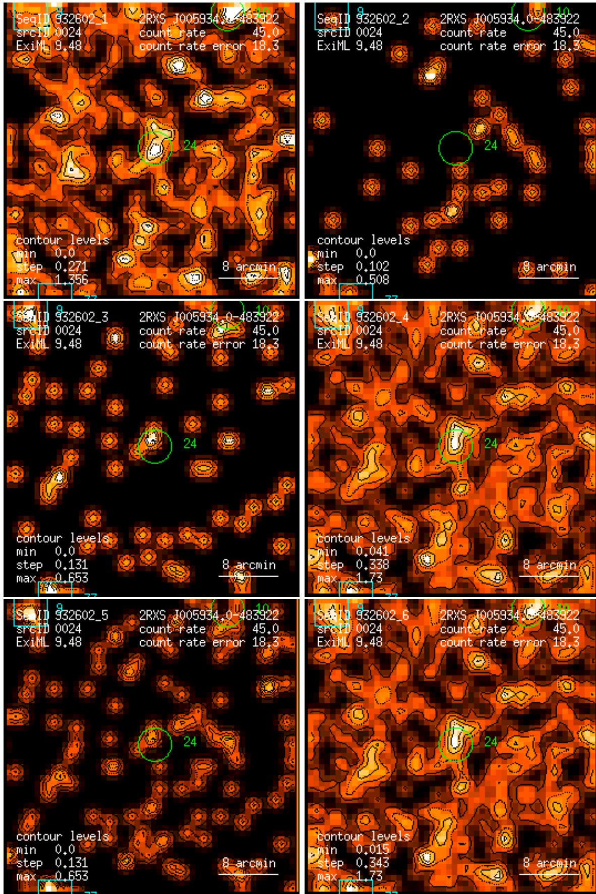
Figure 24: RASS 932602: detection 0024: band rate images, Gaussian filter: (1) PSPC channels 11 – 41, (2) 52 – 90, (3) 91 – 201, (4) 11 – 235, (5) 52 – 201, (6) 11 – 201. Broad band rates in counts/ks. Band rate contour levels in counts/ks/arcmin 2 .
