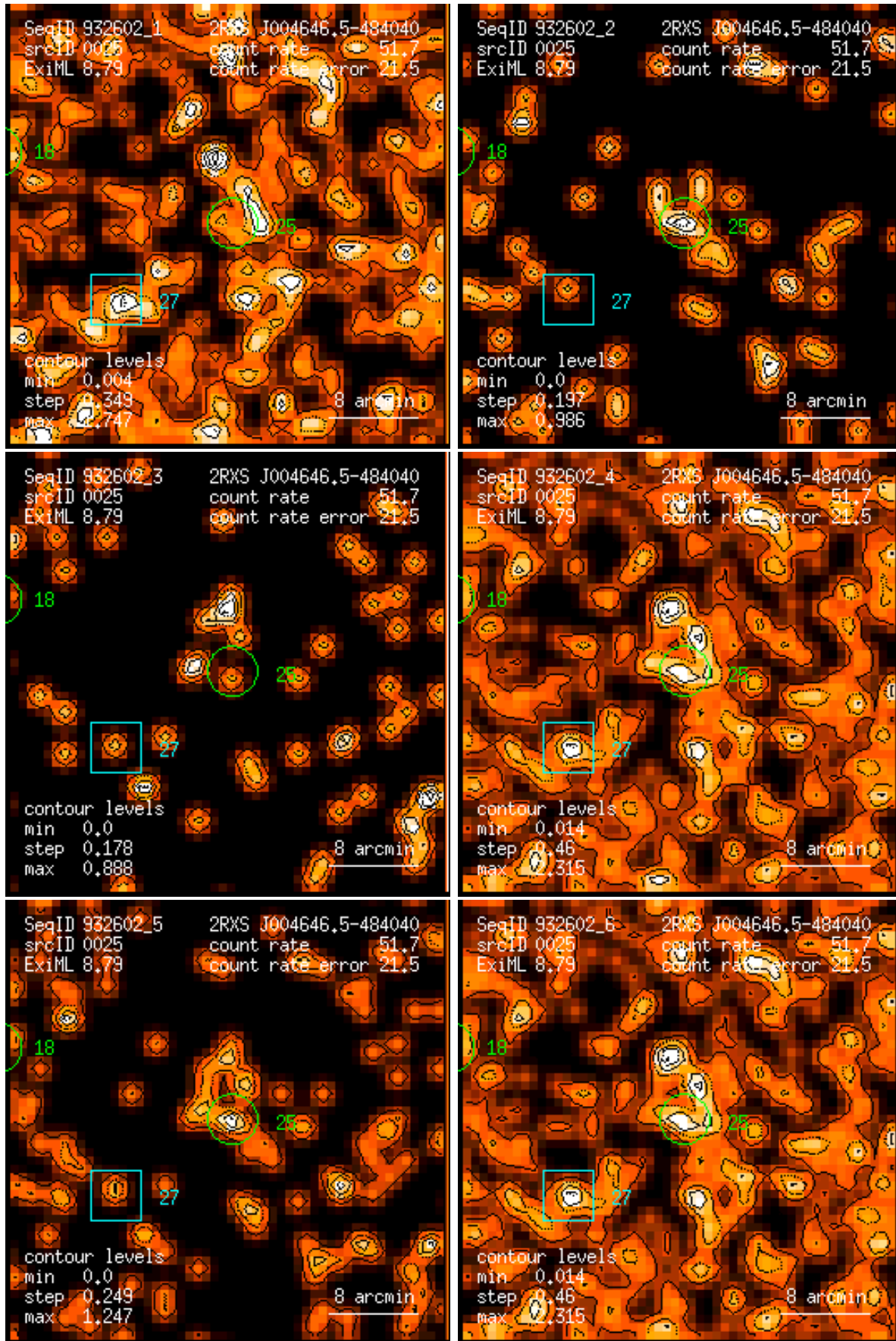
Figure 25: RASS 932602: detection 0025: band rate images, Gaussian filter: (1) PSPC channels 11 – 41, (2) 52 – 90, (3) 91 – 201, (4) 11 – 235, (5) 52 – 201, (6) 11 – 201. Broad band rates in counts/ks. Band rate contour levels in counts/ks/arcmin 2 .
