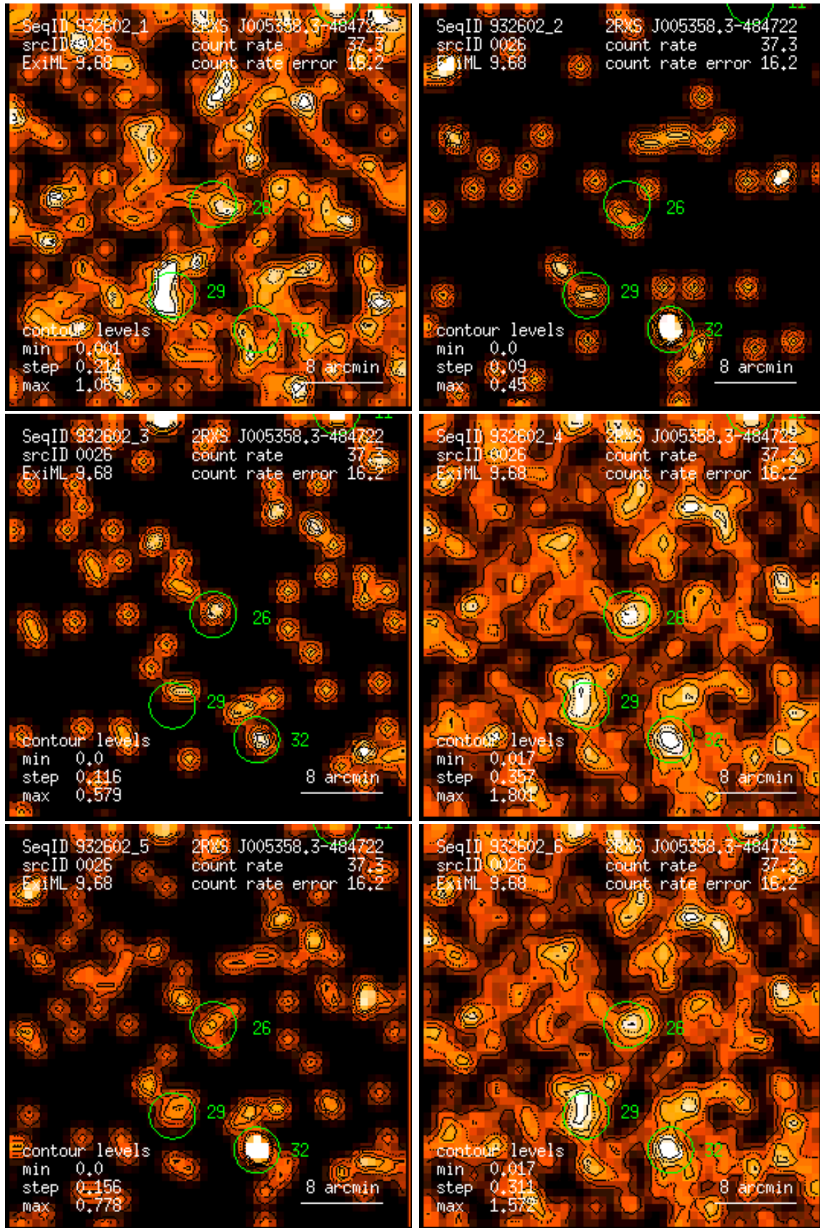
Figure 26: RASS 932602: detection 0026: band rate images, Gaussian filter: (1) PSPC channels 11 – 41, (2) 52 – 90, (3) 91 – 201, (4) 11 – 235, (5) 52 – 201, (6) 11 – 201. Broad band rates in counts/ks. Band rate contour levels in counts/ks/arcmin 2 .
