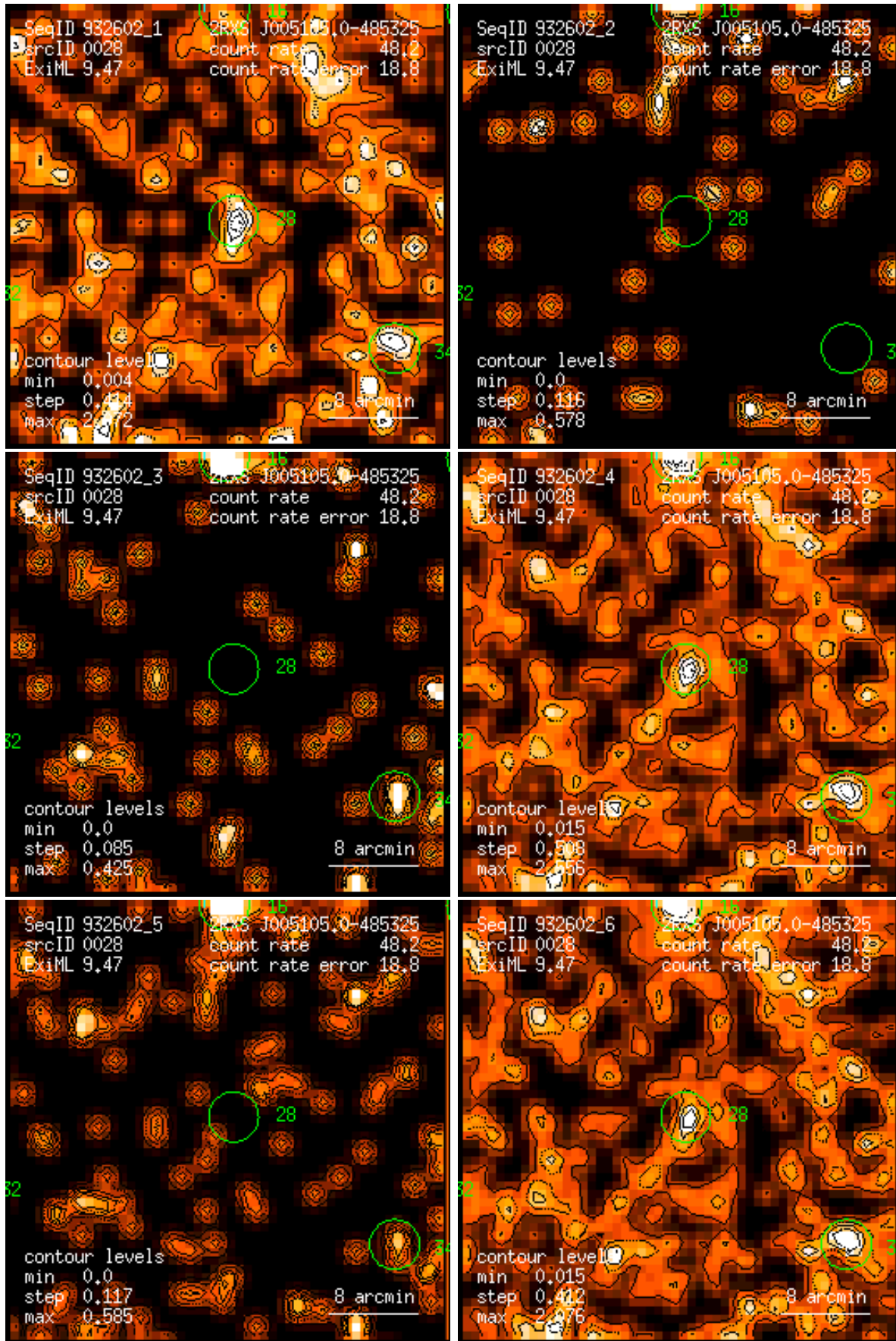
Figure 28: RASS 932602: detection 0028: band rate images, Gaussian filter: (1) PSPC channels 11 – 41, (2) 52 – 90, (3) 91 – 201, (4) 11 – 235, (5) 52 – 201, (6) 11 – 201. Broad band rates in counts/ks. Band rate contour levels in counts/ks/arcmin 2 .
