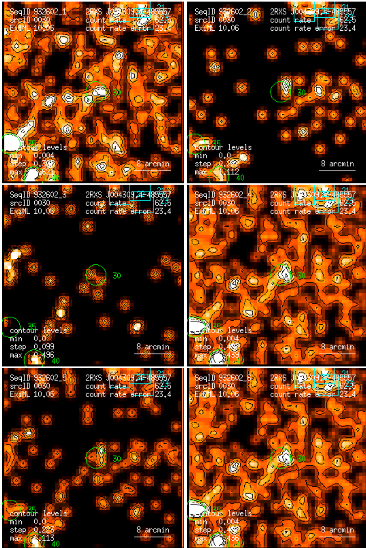
Figure 30: RASS 932602: detection 0030: band rate images, Gaussian filter: (1) PSPC channels 11 – 41, (2) 52 – 90, (3) 91 – 201, (4) 11 – 235, (5) 52 – 201, (6) 11 – 201. Broad band rates in counts/ks. Band rate contour levels in counts/ks/arcmin 2 .
