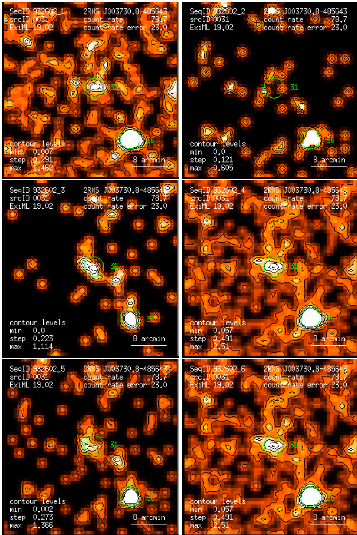
Figure 31: RASS 932602: detection 0031: band rate images, Gaussian filter: (1) PSPC channels 11 – 41, (2) 52 – 90, (3) 91 – 201, (4) 11 – 235, (5) 52 – 201, (6) 11 – 201. Broad band rates in counts/ks. Band rate contour levels in counts/ks/arcmin 2 .
