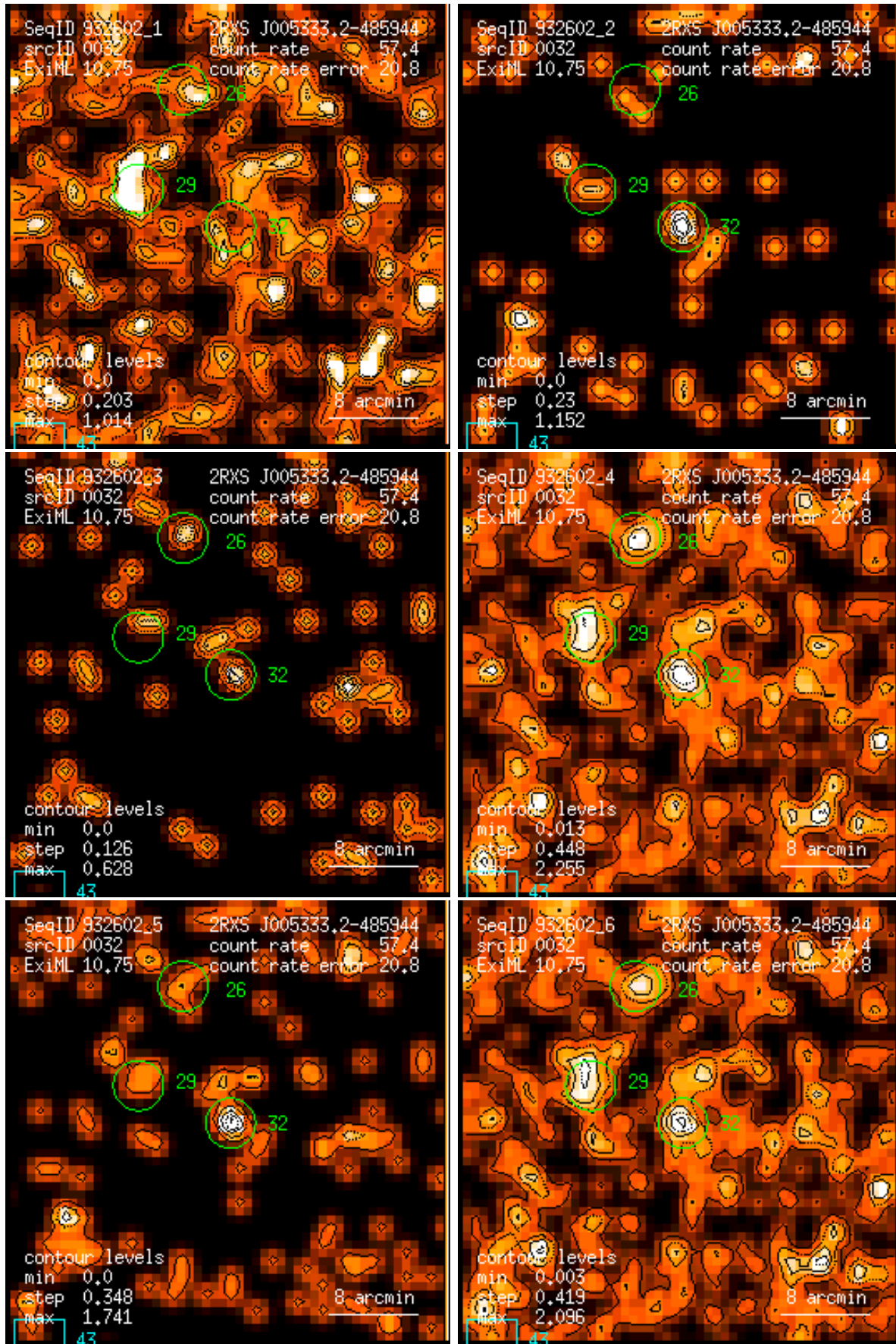
Figure 32: RASS 932602: detection 0032: band rate images, Gaussian filter: (1) PSPC channels 11 – 41, (2) 52 – 90, (3) 91 – 201, (4) 11 – 235, (5) 52 – 201, (6) 11 – 201. Broad band rates in counts/ks. Band rate contour levels in counts/ks/arcmin 2 .
