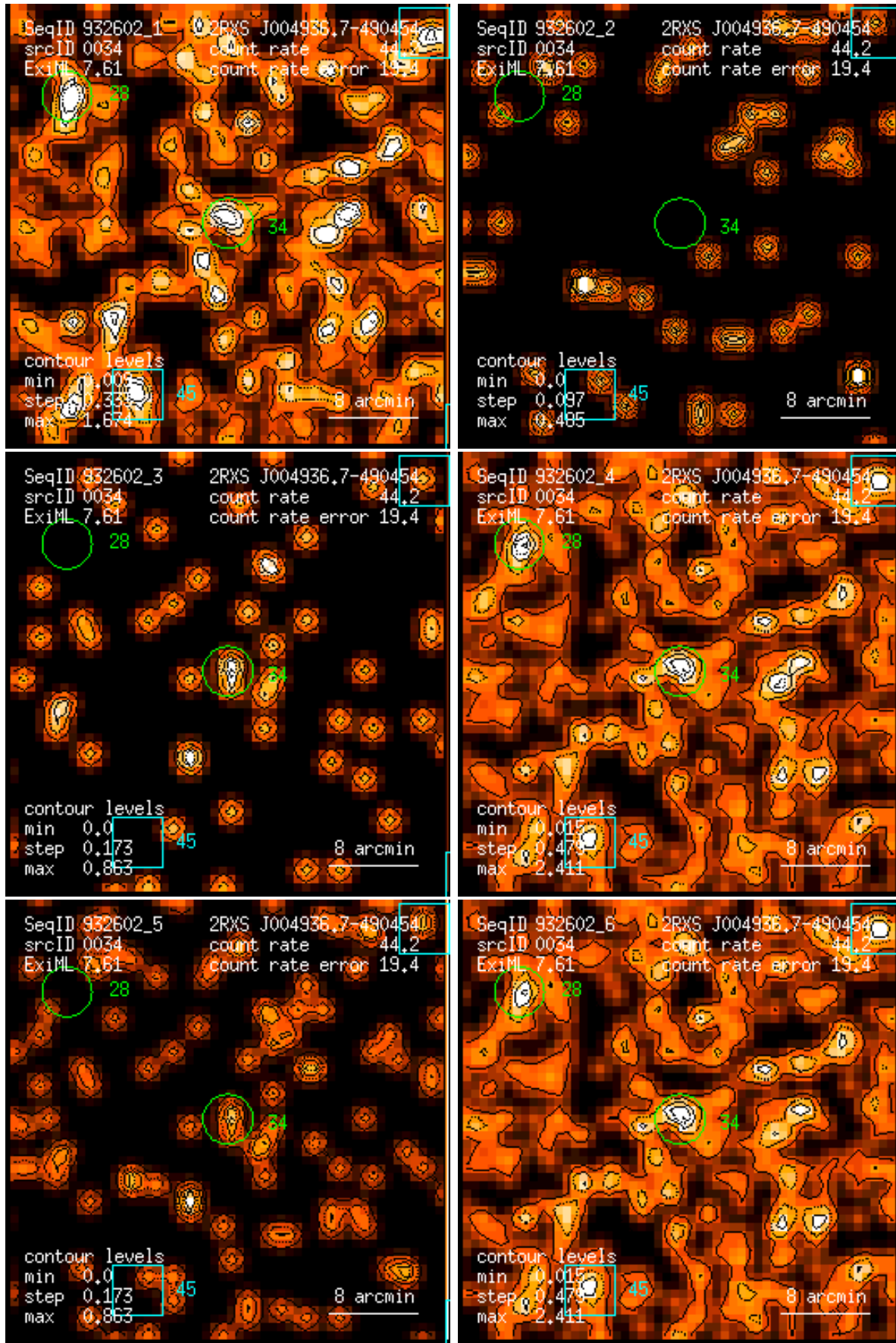
Figure 34: RASS 932602: detection 0034: band rate images, Gaussian filter: (1) PSPC channels 11 – 41, (2) 52 – 90, (3) 91 – 201, (4) 11 – 235, (5) 52 – 201, (6) 11 – 201. Broad band rates in counts/ks. Band rate contour levels in counts/ks/arcmin 2 .
