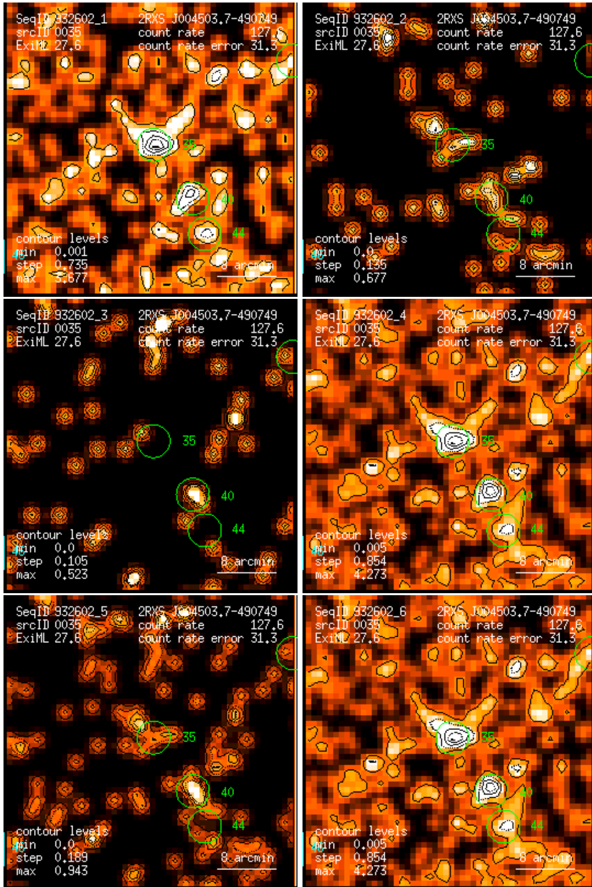
Figure 35: RASS 932602: detection 0035: band rate images, Gaussian filter: (1) PSPC channels 11 – 41, (2) 52 – 90, (3) 91 – 201, (4) 11 – 235, (5) 52 – 201, (6) 11 – 201. Broad band rates in counts/ks. Band rate contour levels in counts/ks/arcmin 2 .
