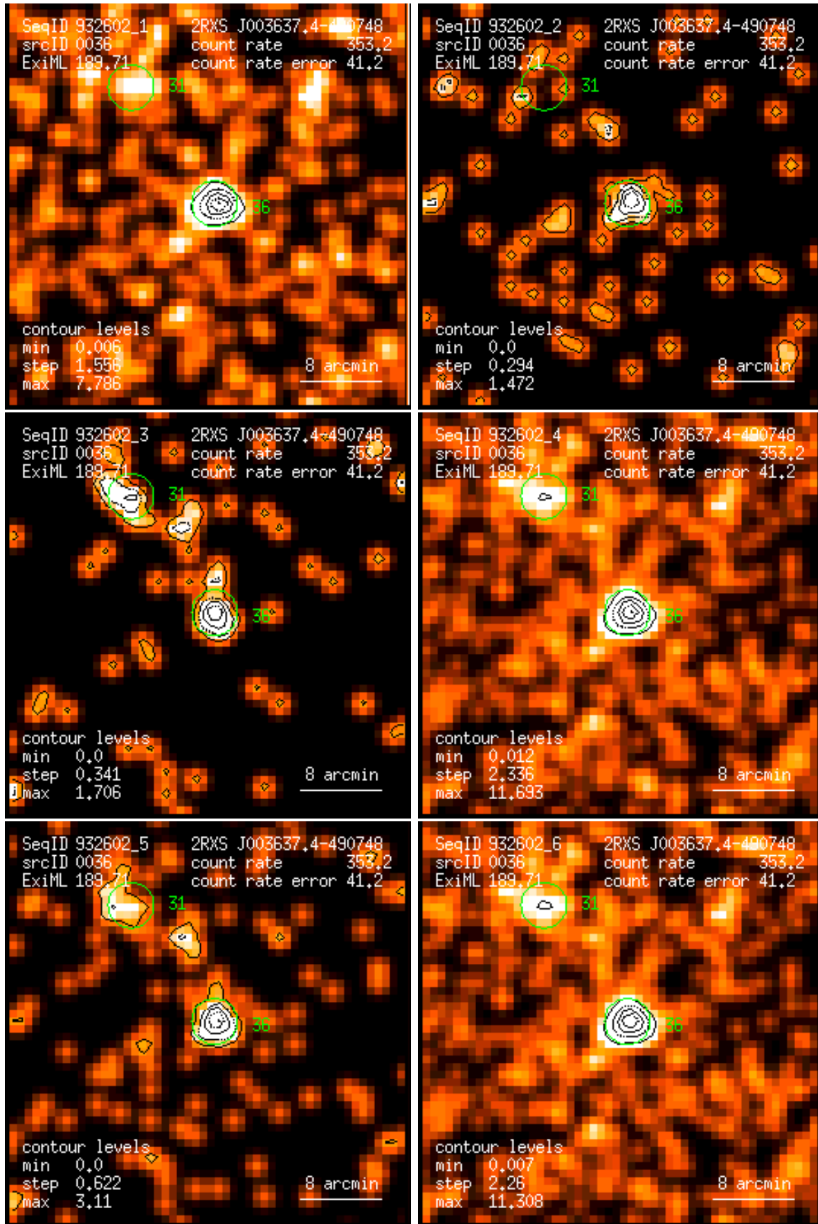
Figure 36: RASS 932602: detection 0036: band rate images, Gaussian filter: (1) PSPC channels 11 – 41, (2) 52 – 90, (3) 91 – 201, (4) 11 – 235, (5) 52 – 201, (6) 11 – 201. Broad band rates in counts/ks. Band rate contour levels in counts/ks/arcmin 2 .
