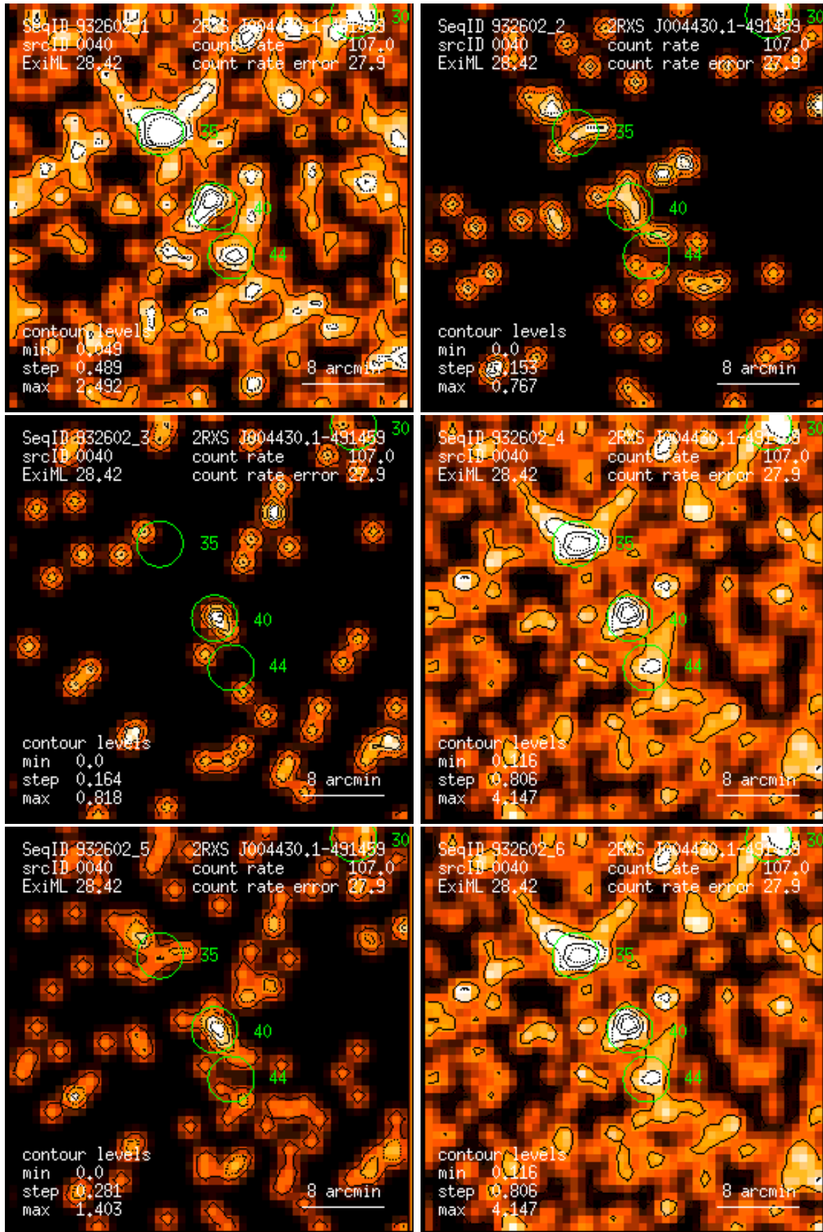
Figure 40: RASS 932602: detection 0040: band rate images, Gaussian filter: (1) PSPC channels 11 – 41, (2) 52 – 90, (3) 91 – 201, (4) 11 – 235, (5) 52 – 201, (6) 11 – 201. Broad band rates in counts/ks. Band rate contour levels in counts/ks/arcmin 2 .
