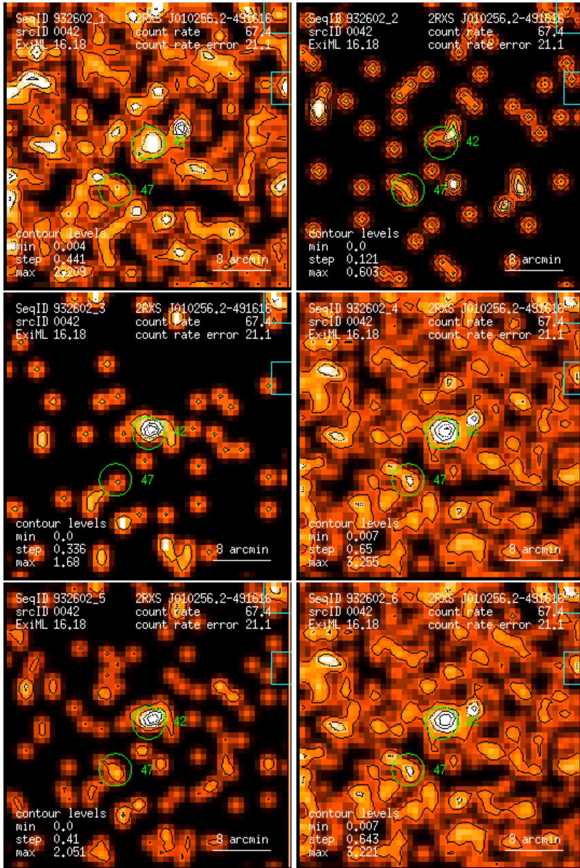
Figure 42: RASS 932602: detection 0042: band rate images, Gaussian filter: (1) PSPC channels 11 – 41, (2) 52 – 90, (3) 91 – 201, (4) 11 – 235, (5) 52 – 201, (6) 11 – 201. Broad band rates in counts/ks. Band rate contour levels in counts/ks/arcmin 2 .
