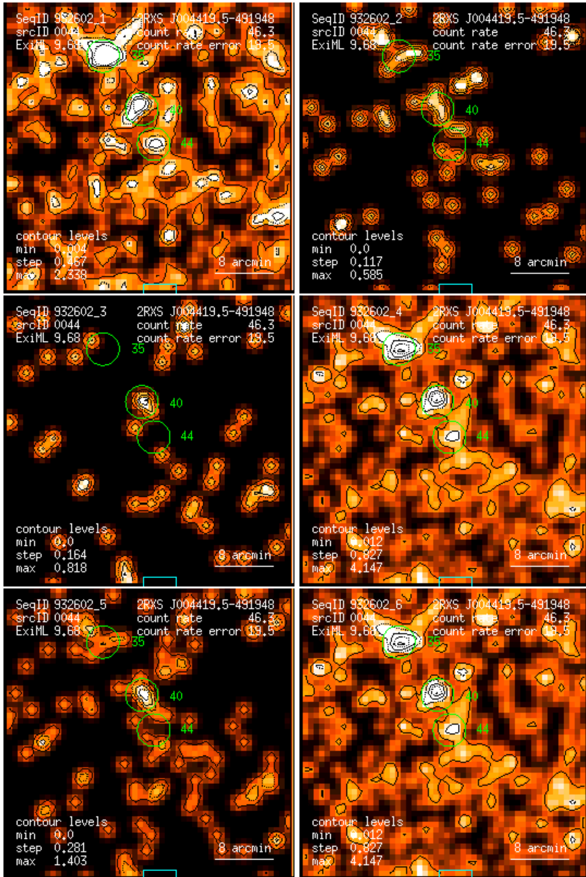
Figure 44: RASS 932602: detection 0044: band rate images, Gaussian filter: (1) PSPC channels 11 – 41, (2) 52 – 90, (3) 91 – 201, (4) 11 – 235, (5) 52 – 201, (6) 11 – 201. Broad band rates in counts/ks. Band rate contour levels in counts/ks/arcmin 2 .
