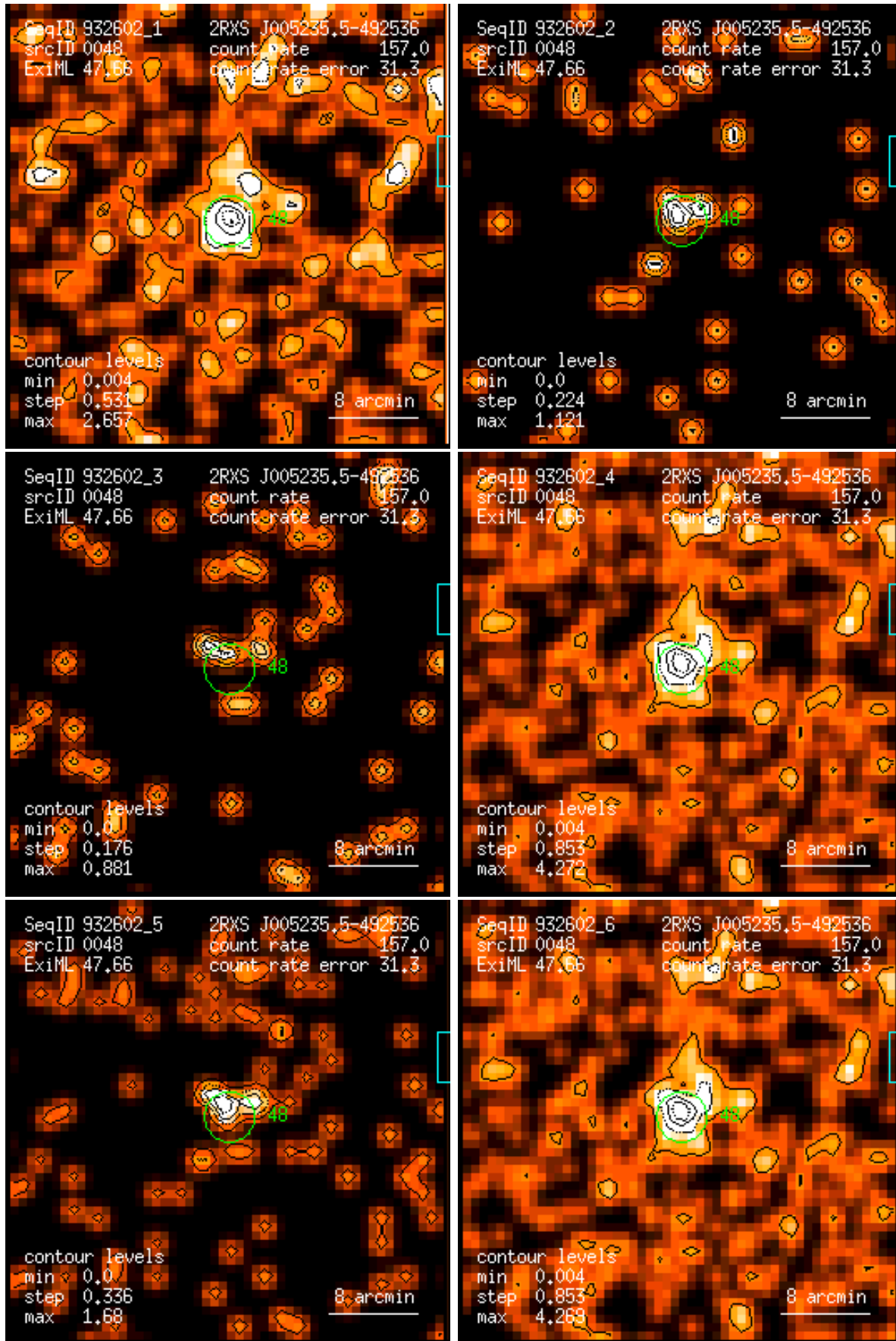
Figure 48: RASS 932602: detection 0048: band rate images, Gaussian filter: (1) PSPC channels 11 – 41, (2) 52 – 90, (3) 91 – 201, (4) 11 – 235, (5) 52 – 201, (6) 11 – 201. Broad band rates in counts/ks. Band rate contour levels in counts/ks/arcmin 2 .
