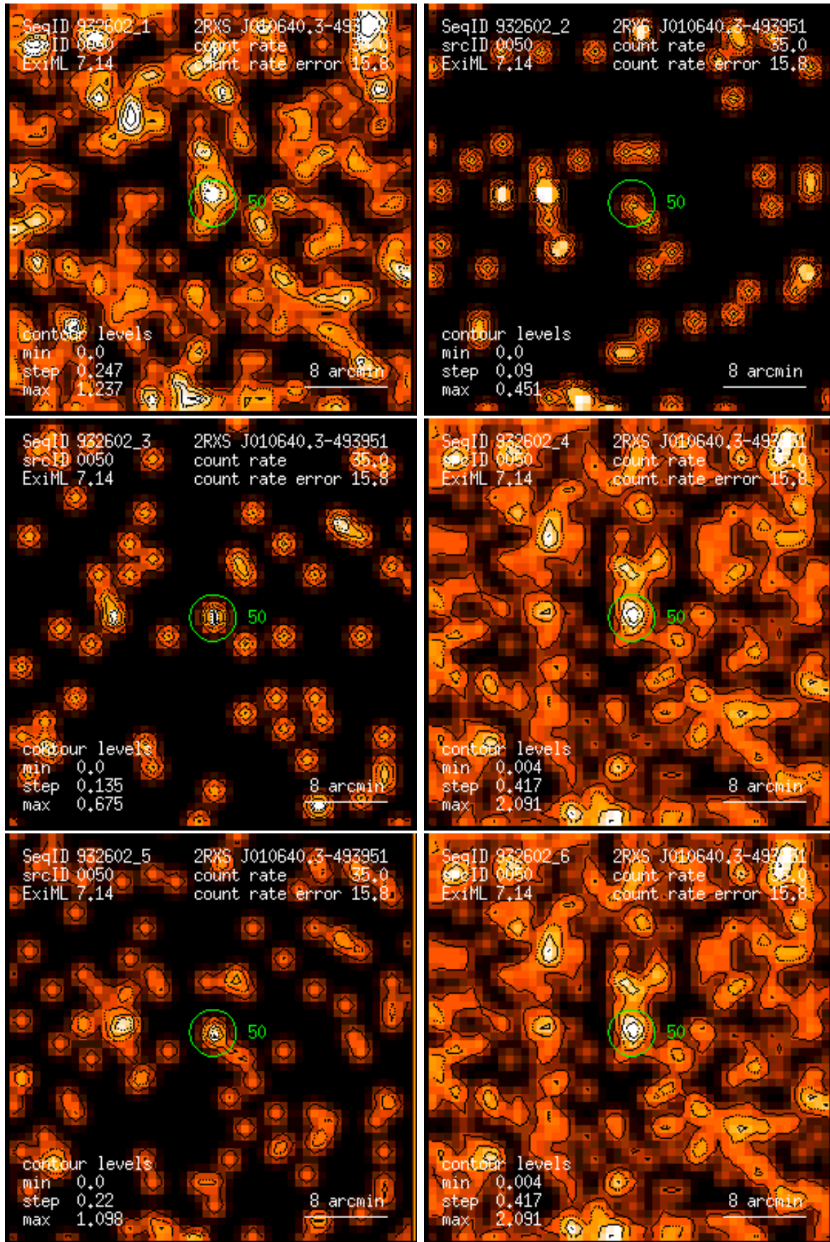
Figure 50: RASS 932602: detection 0050: band rate images, Gaussian filter: (1) PSPC channels 11 – 41, (2) 52 – 90, (3) 91 – 201, (4) 11 – 235, (5) 52 – 201, (6) 11 – 201. Broad band rates in counts/ks. Band rate contour levels in counts/ks/arcmin 2 .
