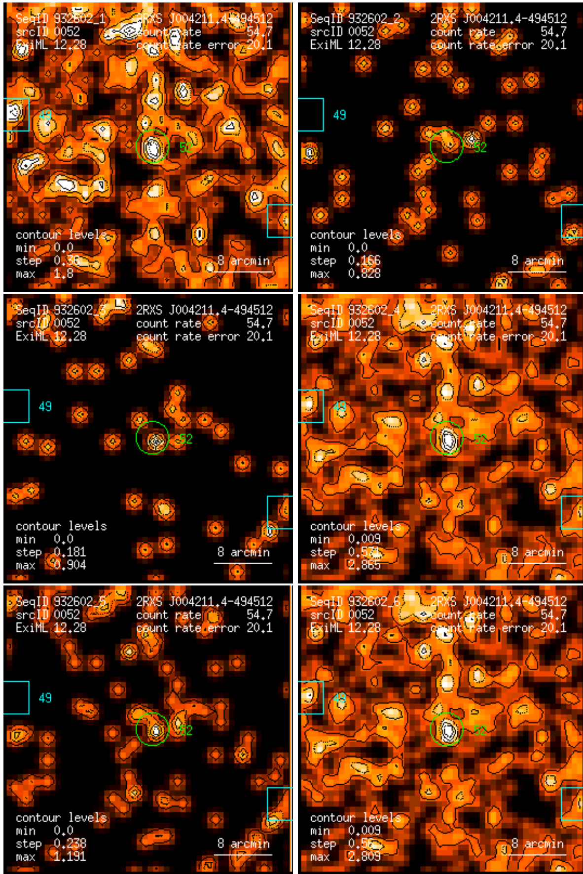
Figure 52: RASS 932602: detection 0052: band rate images, Gaussian filter: (1) PSPC channels 11 – 41, (2) 52 – 90, (3) 91 – 201, (4) 11 – 235, (5) 52 – 201, (6) 11 – 201. Broad band rates in counts/ks. Band rate contour levels in counts/ks/arcmin 2 .
