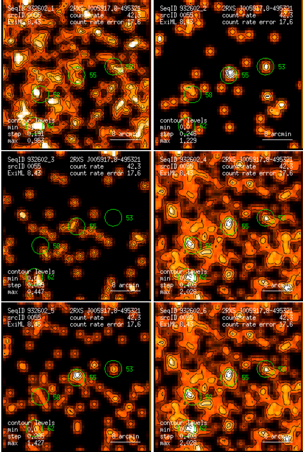
Figure 55: RASS 932602: detection 0055: band rate images, Gaussian filter: (1) PSPC channels 11 – 41, (2) 52 – 90, (3) 91 – 201, (4) 11 – 235, (5) 52 – 201, (6) 11 – 201. Broad band rates in counts/ks. Band rate contour levels in counts/ks/arcmin 2 .
