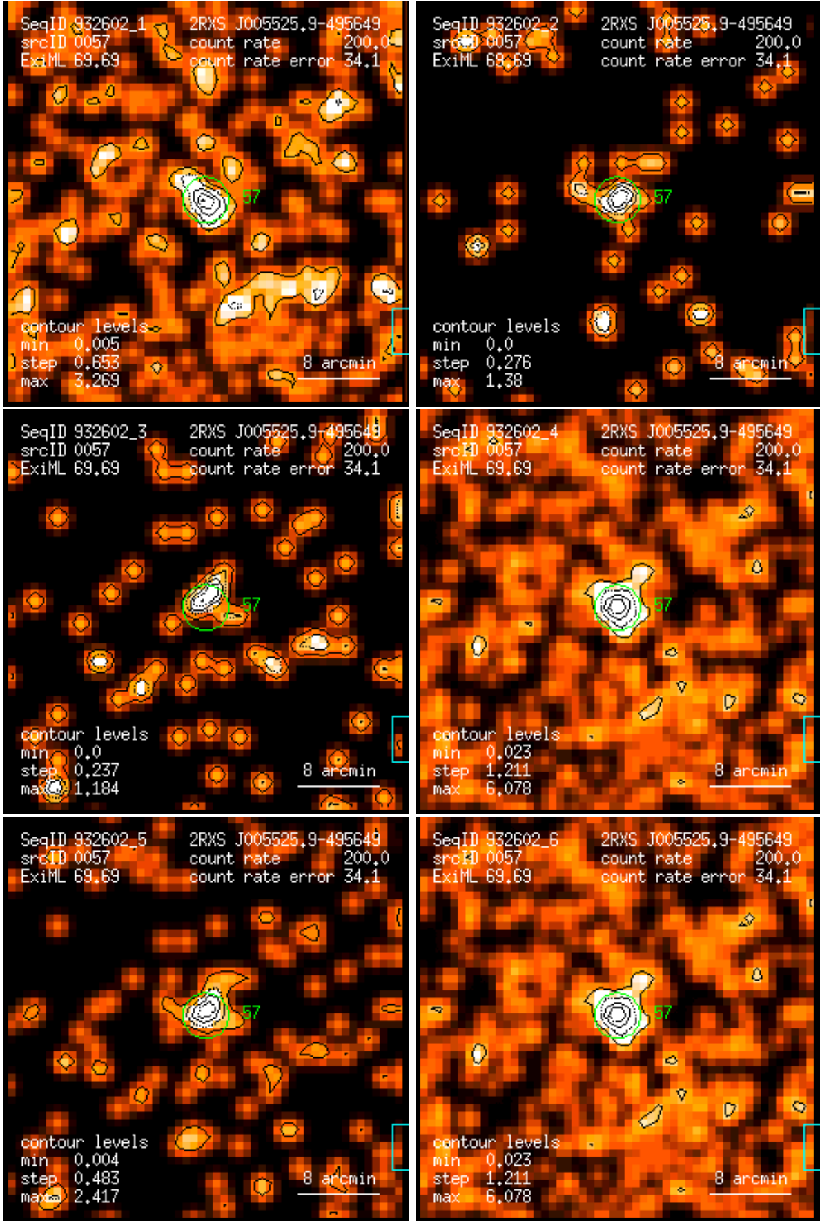
Figure 57: RASS 932602: detection 0057: band rate images, Gaussian filter: (1) PSPC channels 11 – 41, (2) 52 – 90, (3) 91 – 201, (4) 11 – 235, (5) 52 – 201, (6) 11 – 201. Broad band rates in counts/ks. Band rate contour levels in counts/ks/arcmin 2 .
