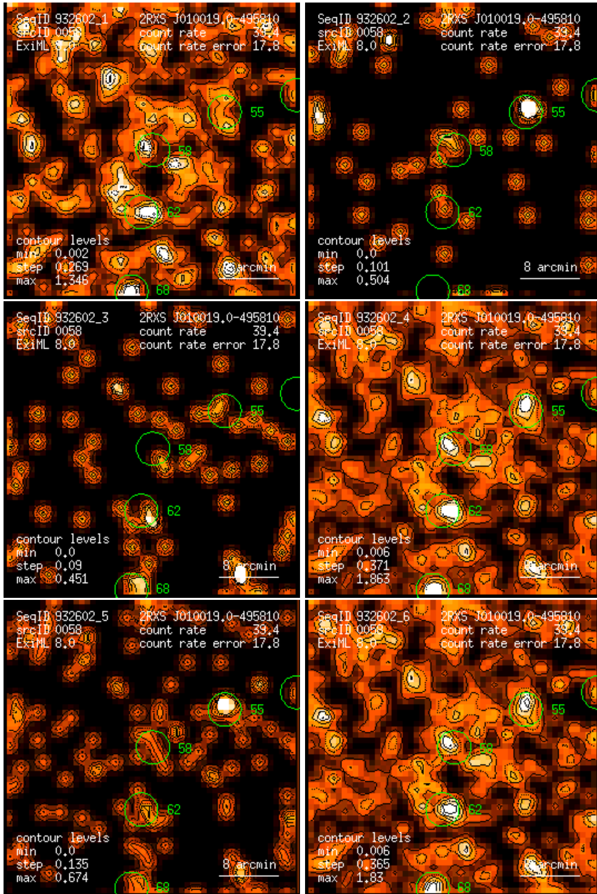
Figure 58: RASS 932602: detection 0058: band rate images, Gaussian filter: (1) PSPC channels 11 – 41, (2) 52 – 90, (3) 91 – 201, (4) 11 – 235, (5) 52 – 201, (6) 11 – 201. Broad band rates in counts/ks. Band rate contour levels in counts/ks/arcmin 2 .
