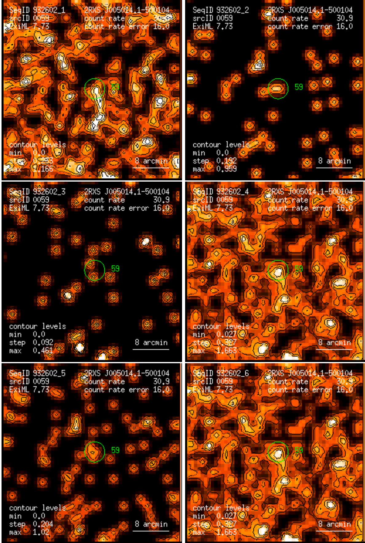
Figure 59: RASS 932602: detection 0059: band rate images, Gaussian filter: (1) PSPC channels 11 – 41, (2) 52 – 90, (3) 91 – 201, (4) 11 – 235, (5) 52 – 201, (6) 11 – 201. Broad band rates in counts/ks. Band rate contour levels in counts/ks/arcmin 2 .
