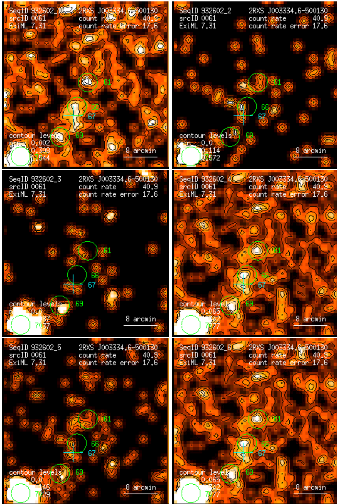
Figure 61: RASS 932602: detection 0061: band rate images, Gaussian filter: (1) PSPC channels 11 – 41, (2) 52 – 90, (3) 91 – 201, (4) 11 – 235, (5) 52 – 201, (6) 11 – 201. Broad band rates in counts/ks. Band rate contour levels in counts/ks/arcmin 2 .
